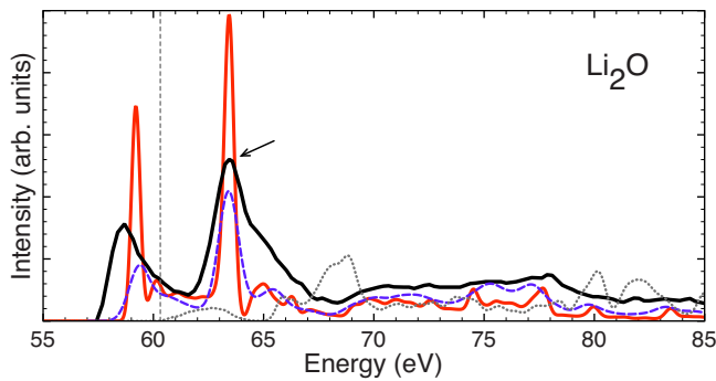
FIG. 4. (Color online) The Li K edge in \text{Li}_2\text{O} . Same notation as Figs. 1 and 2.
