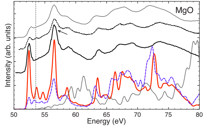
FIG. 1. (Color online) Mg L_{2,3} -edge spectra in MgO. From top to bottom: ELNES data from Ref. 14 with 0.7 (dotted line) and 0.3 eV (dashed line) resolution, and x-ray data from Ref. 15 ( \sim 0.2 eV resolution, full line). Theoretical results are shown below: BSE red (gray) line, supercell blue (dark gray) dashed line, and RPA dotted gray line. The vertical dashed line marks the RPA onset.
