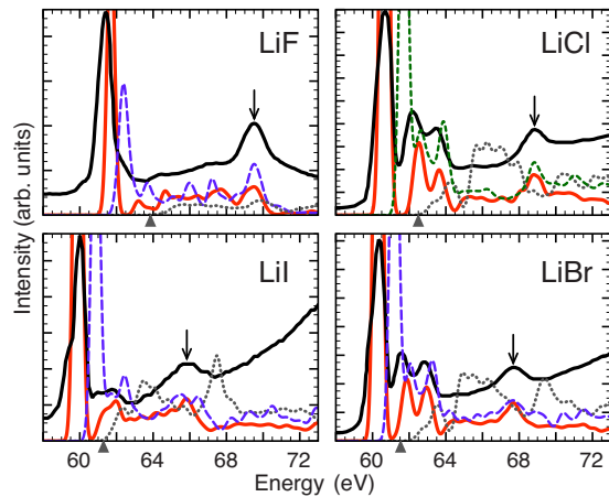
FIG. 2. (Color online) The Li K edge in the lithium halides LiF, LiCl, LiBr, and LiI comparing experiment (full line) (Ref. 18) and theoretical results; BSE red (gray) line, DFT calculations for 64 atoms dashed blue (dark gray) line and in the case of LiCl 128 atoms short-dashed green (dark gray) line, and RPA dotted gray line. The triangles mark the RPA onset.
