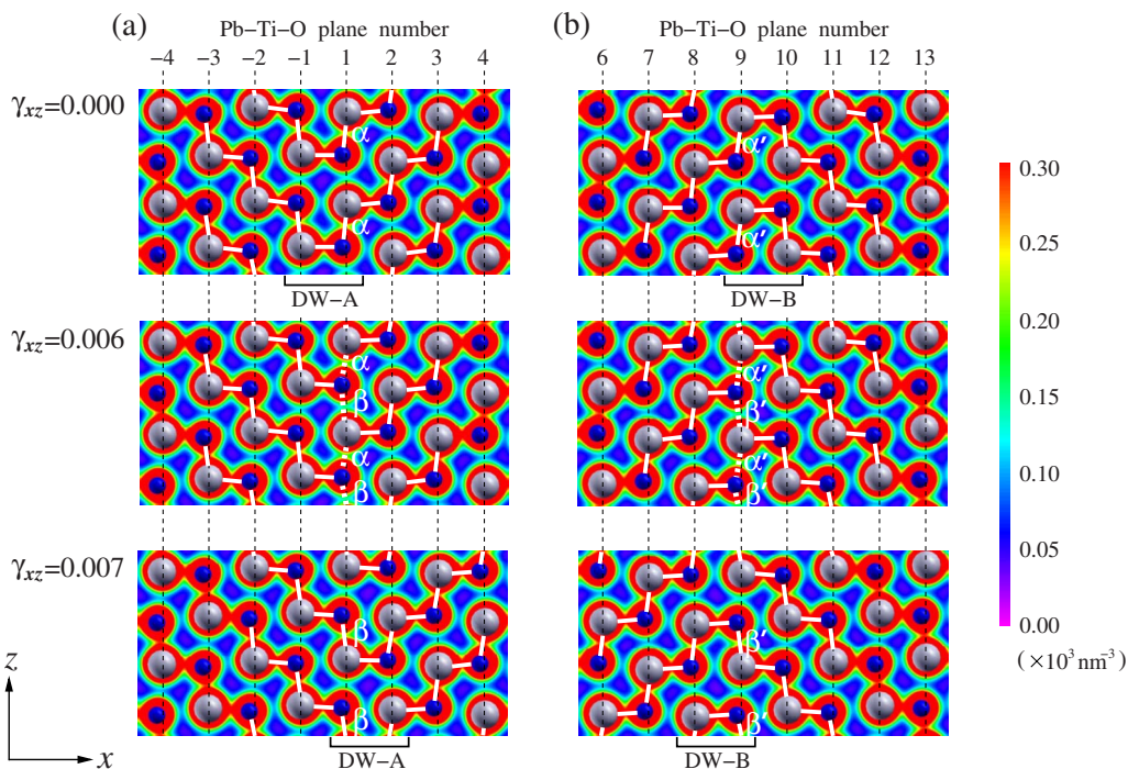
FIG. 8. (Color online) Change in atomistic configurations and charge density distributions near (a) DW-A and (b) DW-B projected on the \text{PbO} (010) plane of the N=18 model under shear deformation. Gray and blue spheres are Pb and O atoms, respectively. The Pb-O bonds around the DWs are drawn with white lines.
