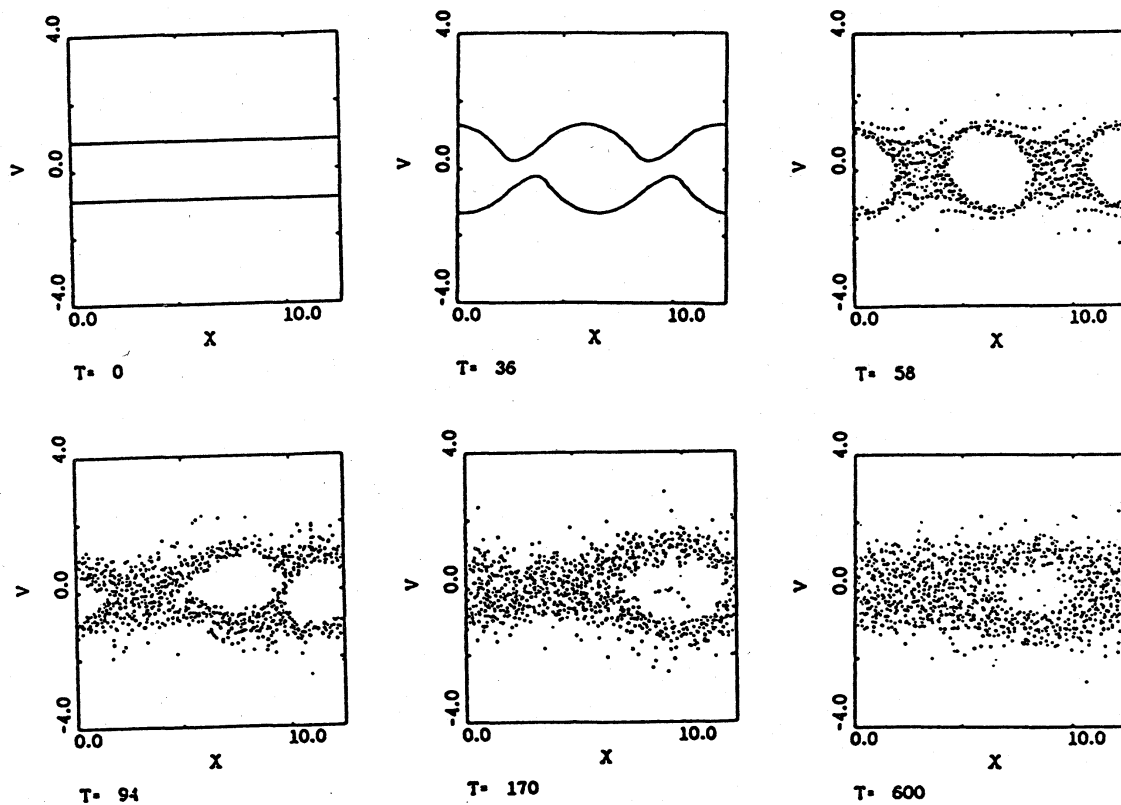
Fig. A typical evolution of 1260 sheets in the phase space. The V axis is the velocity axis and the X axis is the position axis. Time T is scaled by the plasma frequency.
