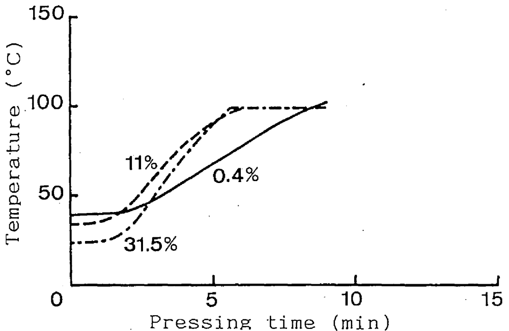
Fig.2.4 The effect of moisture content of mat before pressing on the core temperature of mats along the thickness as a function of time during hot-pressing.
