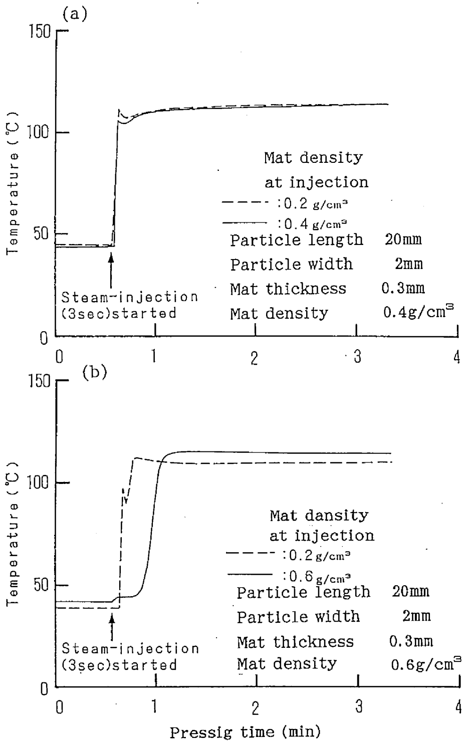
Fig.3.4 Effect of mat density at injection on temperature behavior of mat core.
