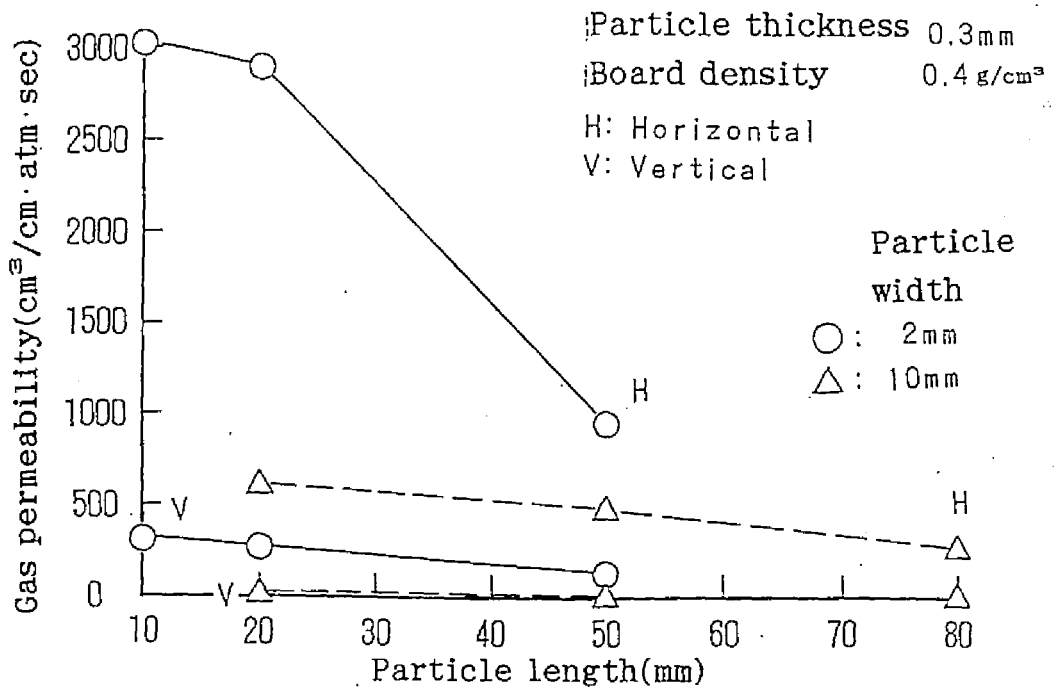
Fig.3.6 Effect of particle length on gas permeability of boards.
