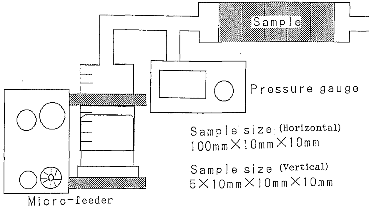
Fig.3.5 System for measuring air permeability.
