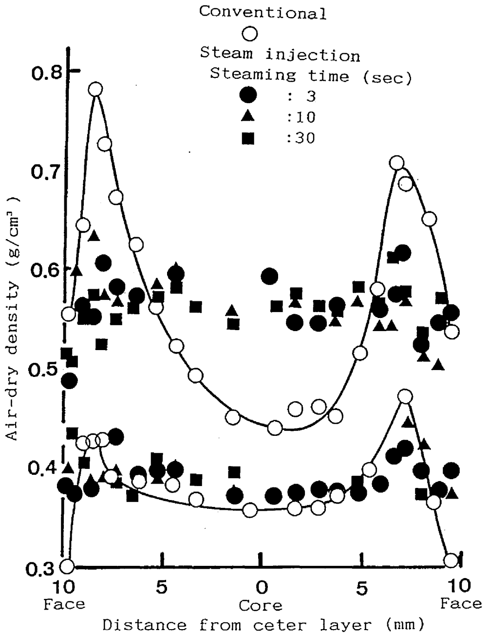
Fig.4.1 Density profiles through the thickness of boards
