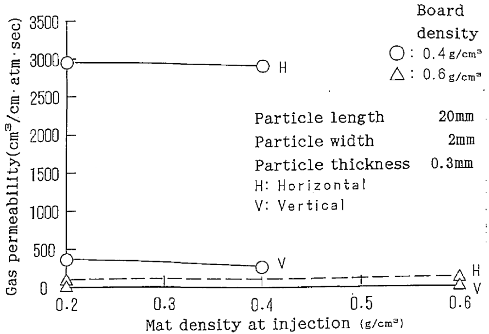
Fig.3.8 Effect of mat density at injection on gas permeability of boards.
