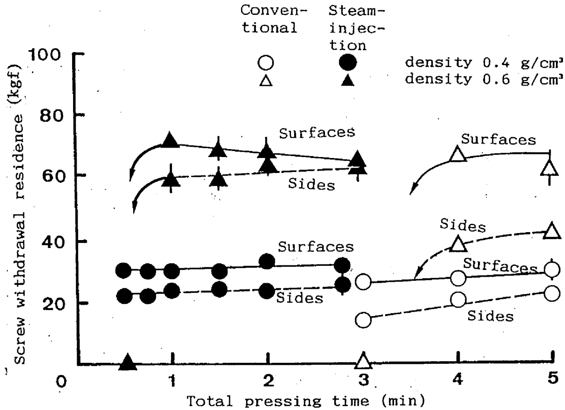
Fig.4.17 Relationships between total pressing time and screw withdrawal residence.
