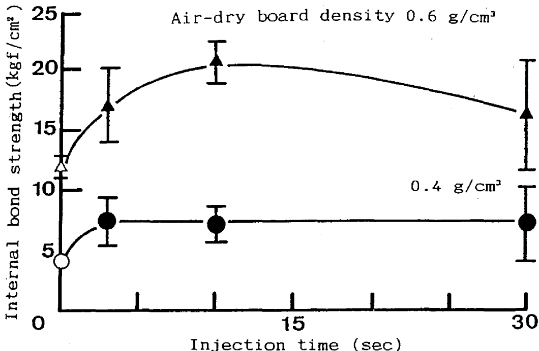
Fig.4.3 Relationships between steam-injection time and internal bond strength.
