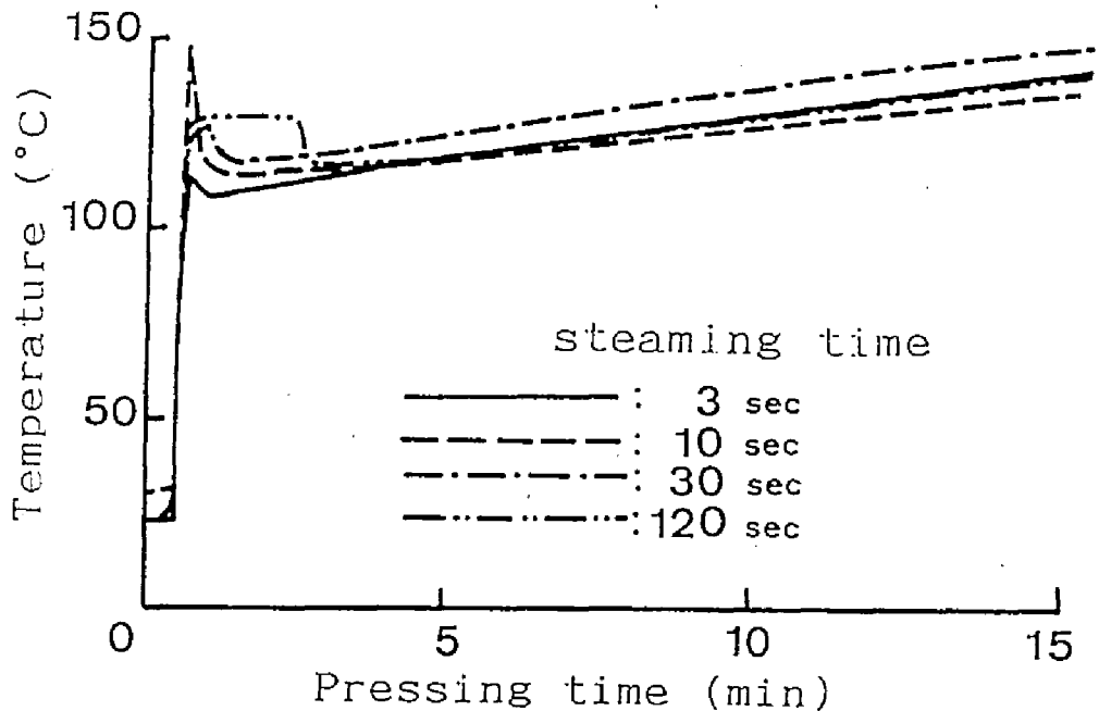
Fig.2.6 The effect of steam-injection time on the core temperature of mats.
