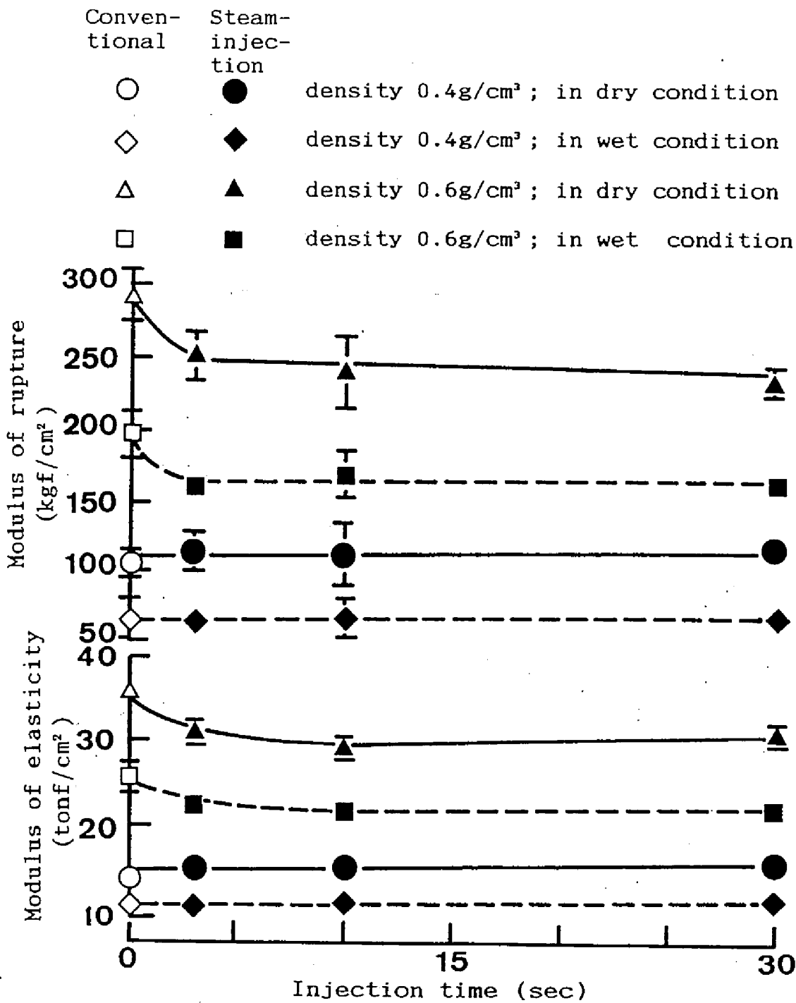
Fig.4.2 Relationships between steam-injection time and modulus of elasticity and modulus of rupture in dry and wet condition.
