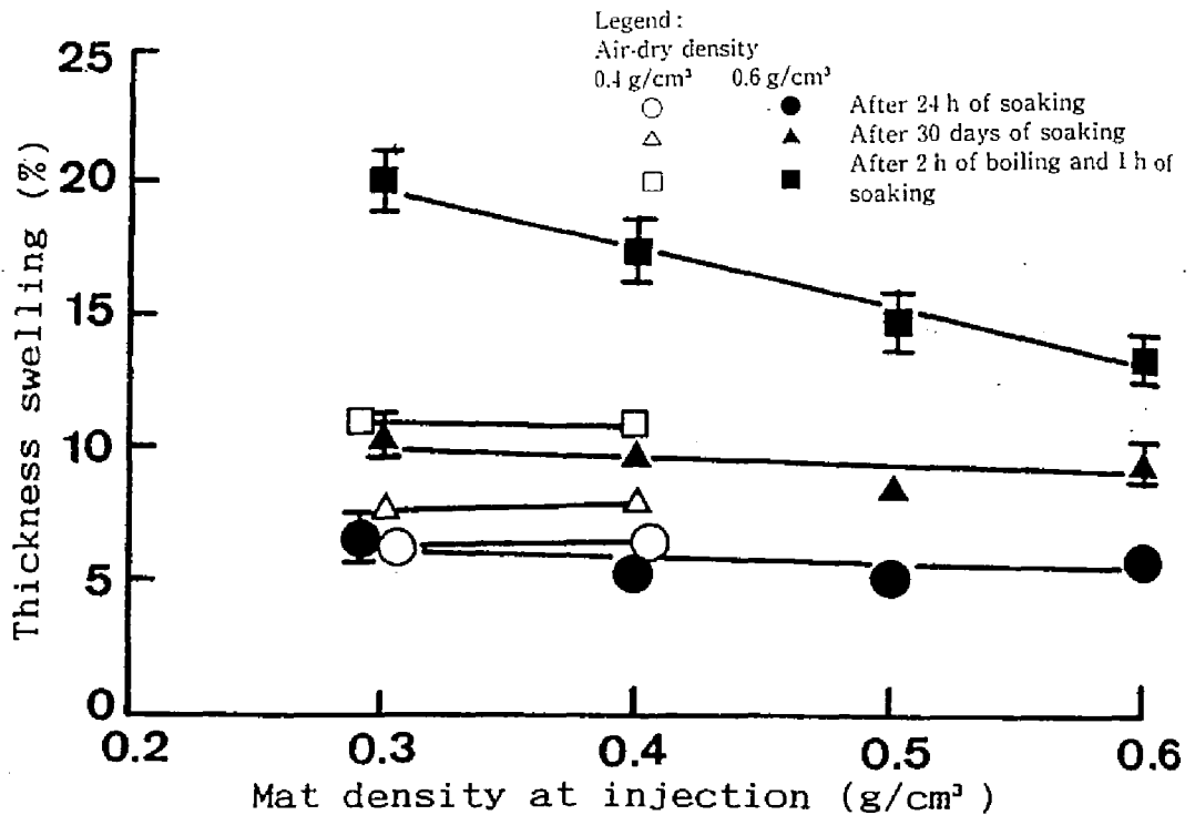
Fig.4.7 Relationships between mat density at steam-injection and thickness swelling.
