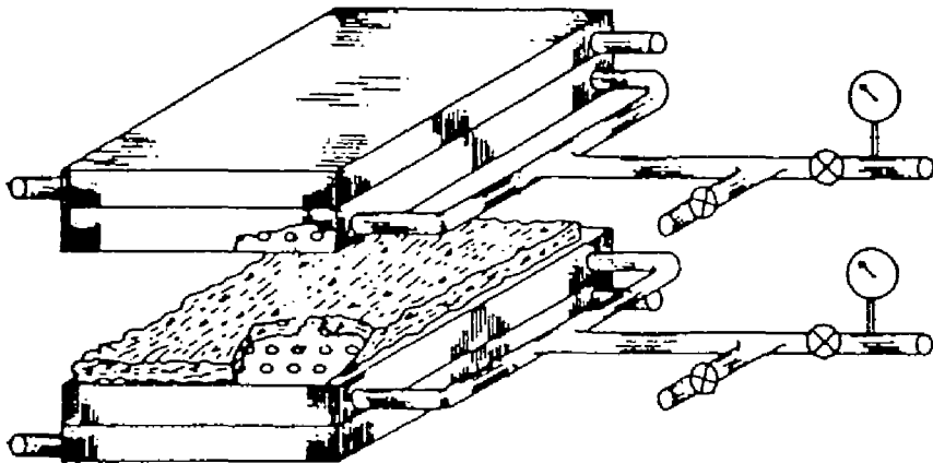
Fig. 1.3 Schematic of an Unsealed Steam Press.
