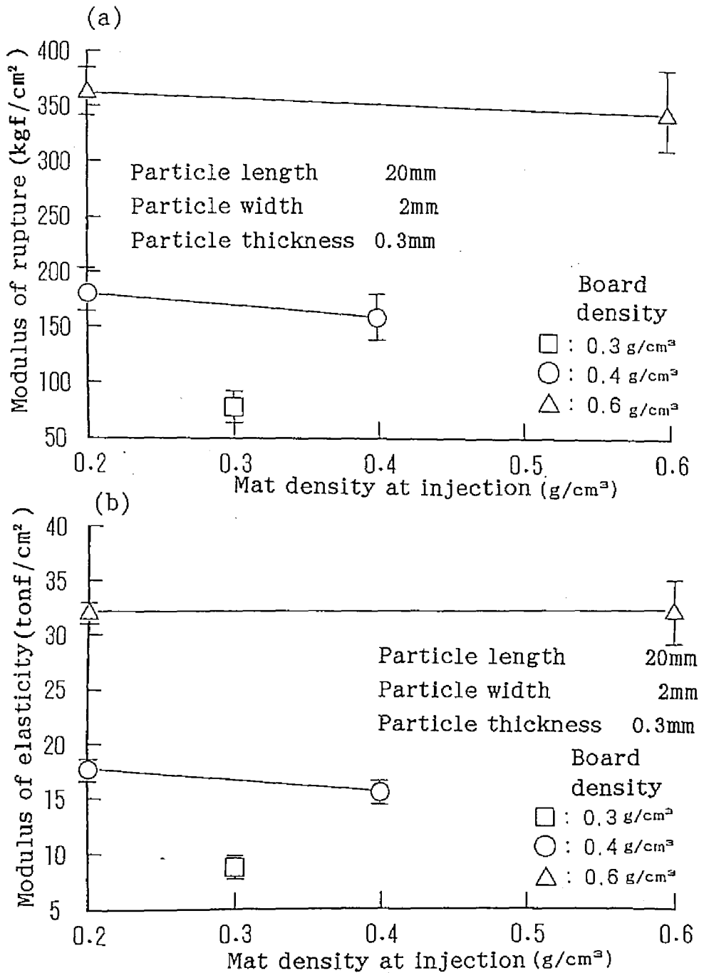
Fig.4.12 Effect of mat density at injection on MOR and MOE.
