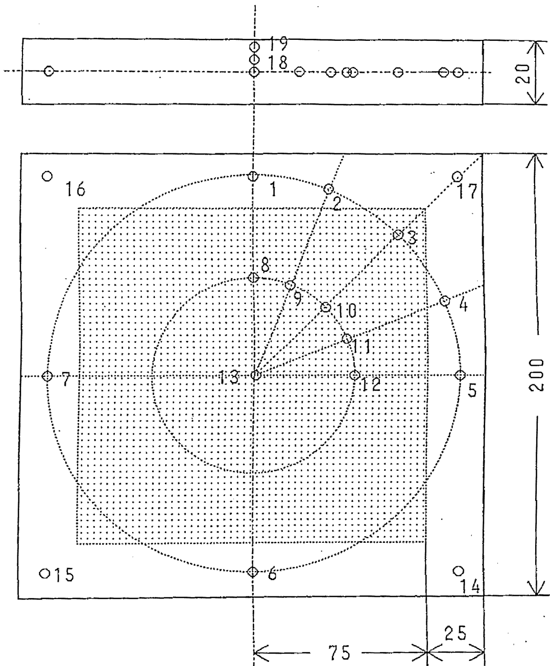
Fig.3.1 Location of thermocouples in mat. Note: The mesh shows an area of steam perforations.
