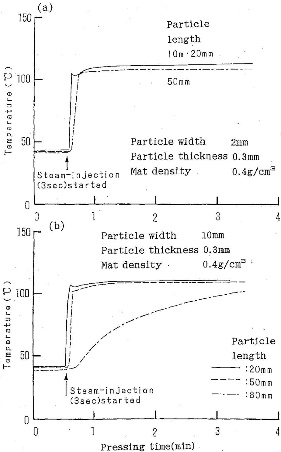
Fig.3.2 Effect of particle length on temperature behavior of mat core.
