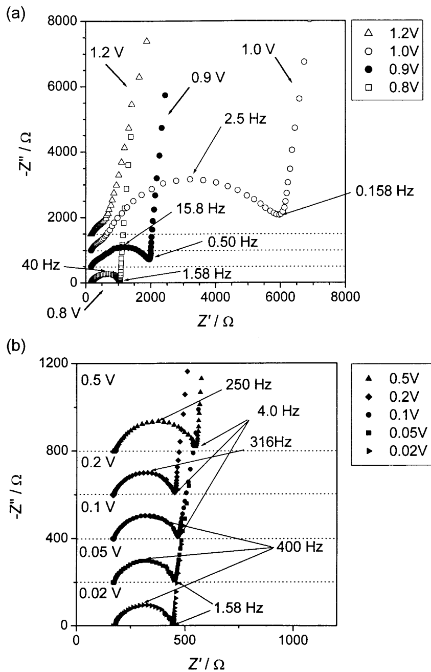
Fig. 9.4. Nyquist plots of carbonaceous thin-film electrode prepared at applied rf power of 10 W in 1 mol dm -3 LiClO 4 /EC+DEC (1:1). (a) Electrode potential is kept at 0.8, 0.9, 1.0, and 1.2 V vs. Li/Li + . (b) Electrode potential is kept at 0.02, 0.05, 0.1, 0.2 and 0.5 V vs. Li/Li + .
