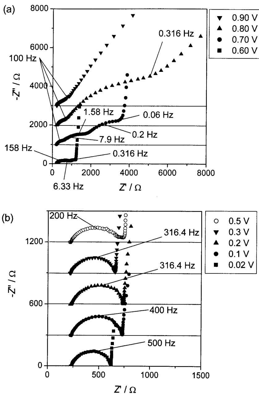
Fig. 9.5. Nyquist plots of carbonaceous thin-film electrode prepared at applied rf power of 50 W in 1 mol dm -3 LiClO 4 /EC+DEC (1:1). (a) Electrode potential is kept at 0.6, 0.7, 0.8, and 0.9 V vs. Li/Li + . (b) Electrode potential is kept at 0.02, 0.1, 0.2, 0.3 and 0.5 V vs. Li/Li + .
