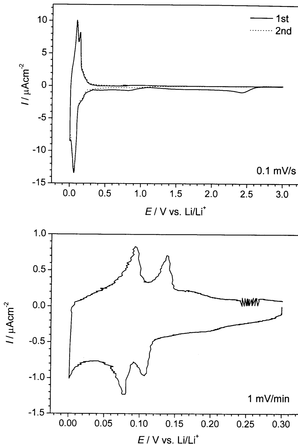
Fig. 4.4. Cyclic voltammograms of carbonaceous thin-film electrode prepared at 10 W in 1 \text{ mol dm}^{-3} \text{ LiClO}_4/\text{EC}+\text{DEC} (1:1). Sweep rate; (top) 0.1 mV/s, and (bottom) 1 mV/min.
