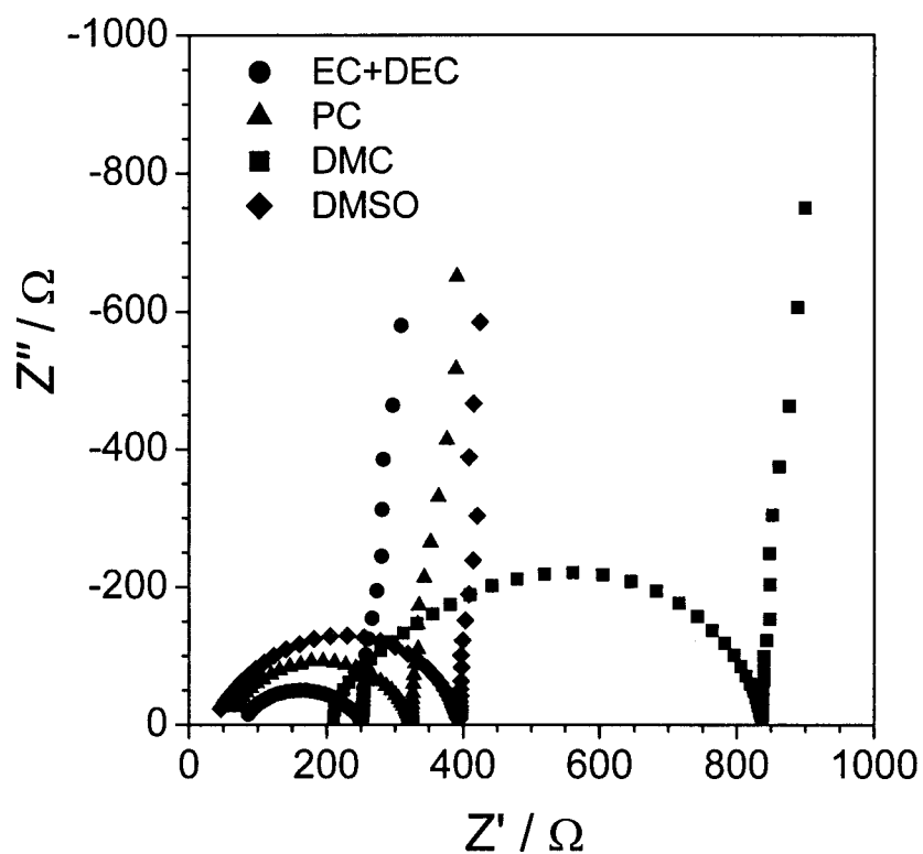
Fig. 8.7. Nyquist plots of carbonaceous thin-film electrodes with SEI formed from EC obtained in various electrolytes at 0.1 V. Electrolytes are 1 \text{ mol dm}^{-3} \text{ LiClO}_4/\text{EC+DEC} , 1 \text{ mol dm}^{-3} \text{ LiClO}_4/\text{PC} , 1 \text{ mol dm}^{-3} \text{ LiClO}_4/\text{DMC} , and 1 \text{ mol dm}^{-3} \text{ LiCF}_3\text{SO}_3/\text{DMSO} .
