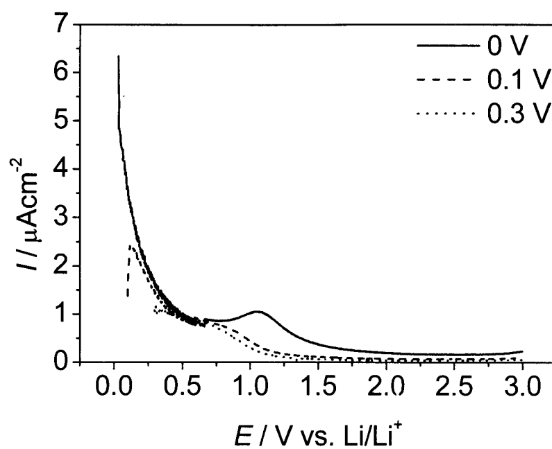
Fig. 2.8. Linear sweep voltammograms (2nd sweep) of carbonaceous thin-film electrodes prepared by plasma CVD in 1 \text{ mol dm}^{-3} \text{LiClO}_4/\text{EC}+\text{DEC} (1:1). Applied rf power; 10 W. Sweep rate; 0.1 mV/s.
