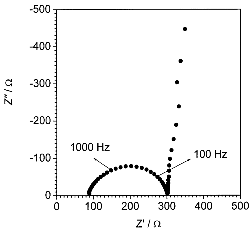
Fig. 8.2. Typical Nyquist plot of carbonaceous thin-film electrode obtained in 1 \text{ mol dm}^{-3} \text{ LiClO}_4/\text{EC}+\text{DEC} at 0.05 \text{ V} .
