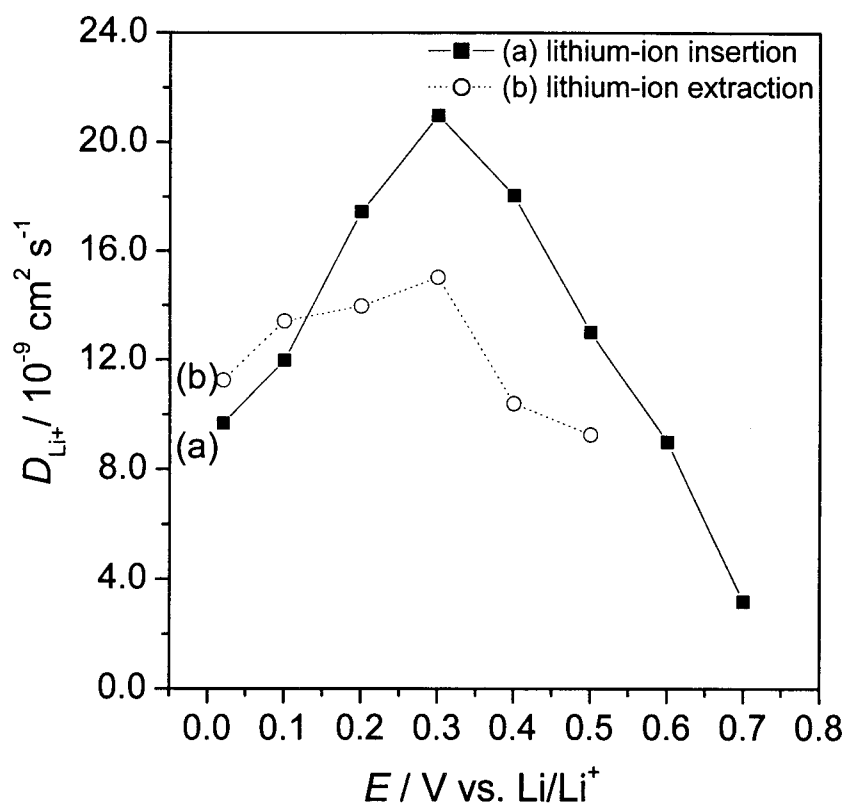
Fig. 7.5. Potential dependence of apparent diffusion coefficient D_{\text{Li}^+} through carbonaceous thin-film electrode prepared at applied rf power of 10 W.
