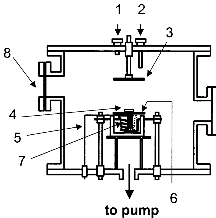
Fig. 1.1. Schematic image of rf reactor for the plasma CVD apparatus. 1; Ar inlet, 2; C 2 H 2 inlet, 3; rf electrode, 4; substrate, 5; thermocouple, 6; ground electrode, 7; tungsten heater, 8; view port.
