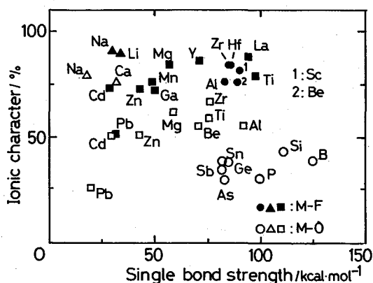
Fig. 3. The ionic character (eq. 1) for metal-fluorine bonds (M-F, filled symbols) and metal-oxygen ones (M-O, open symbols) as a function of their single bond strength. Circles: network formers; triangles: intermediates; squares: network modifiers after Sun 21) and Baldwin and Mackenzie. 22)
