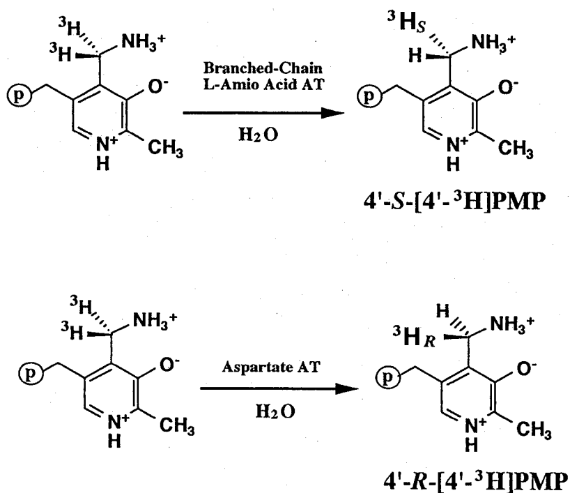
Figure 5. Preparation of (4'\text{-S})\text{-[4'-}^3\text{H]PMP} and (4'\text{-R})\text{-[4'-}^3\text{H]PMP} .
