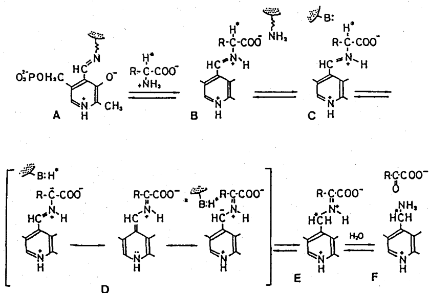
Figure 1. Reaction mechanism of aminotransferase.
