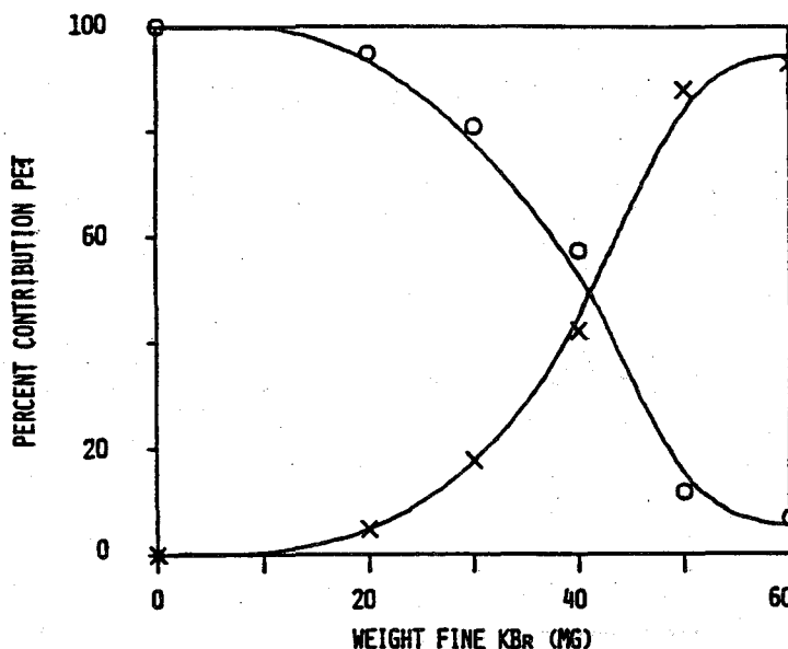
Figure 5. Percent contribution of the 29.5 \mu\text{m} -thick poly (ethylene terephthalate) substrate (O) and the 1.5 \mu\text{m} -thick poly (vinylidene fluoride) overlayer (X) to the composite spectra in the CH stretching region as a function of the weight of the fine (75 \mu\text{m} ) KBr overlayer.
