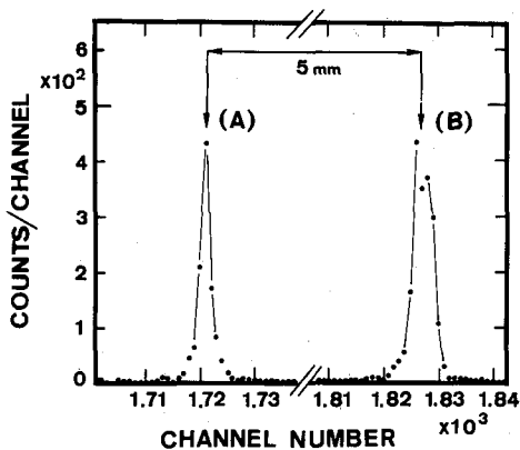
Fig.7. The position spectrum observed with well-collimated x-ray beams. The peak labeled as (A) is obtained with a 25\text{-}\mu\text{m} wide slit. For comparison, the peak, labeled as (B), observed with a 100\text{-}\mu\text{m} wide slit is also shown. The position resolution for the peak A is \sim 100\ \mu\text{m} and that for the peak B is \sim 190\ \mu\text{m} .
