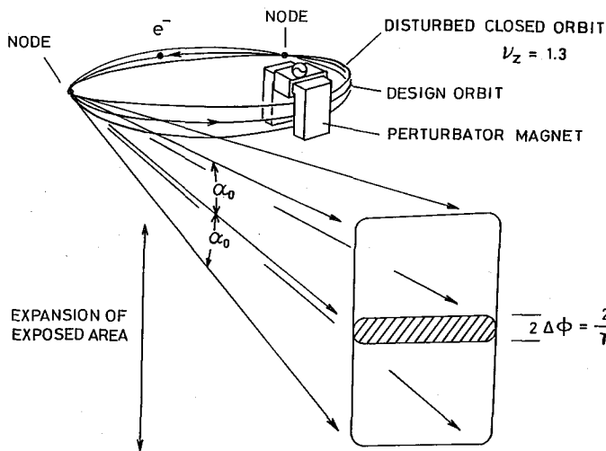
Fig. 11. Expansion of the exposed area of SR by the use of vertically undulating beam near a node. The tilt angle varies between \alpha_0 and \alpha_0 + \Delta\alpha .
