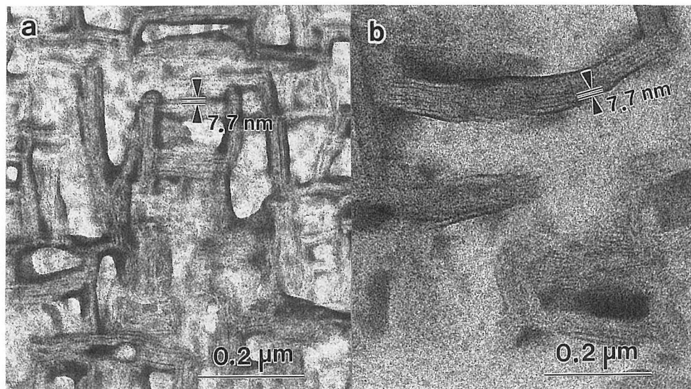
Fig. 6. Edge-on crystals of (\text{CH}_2)_{120} stained with \text{RuO}_4 . (a) Monoclinic (\text{CH}_2)_{120} grown at 60^\circ\text{C} on \text{NaCl} from a solution. (b) Orthorhombic (\text{CH}_2)_{120} prepared by annealing the monoclinic (\text{CH}_2)_{120} on \text{NaCl} at 110^\circ\text{C} for 60 minutes.
