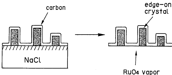
Fig. 2. Preparation procedure of edge-on crystals stained with RuO 4 .
