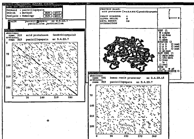
Fig. 5. Comparison of penicillopepsin against endothiapepsin. 3-D graphics of penicillopepsin is also displayed in the upper right window.
