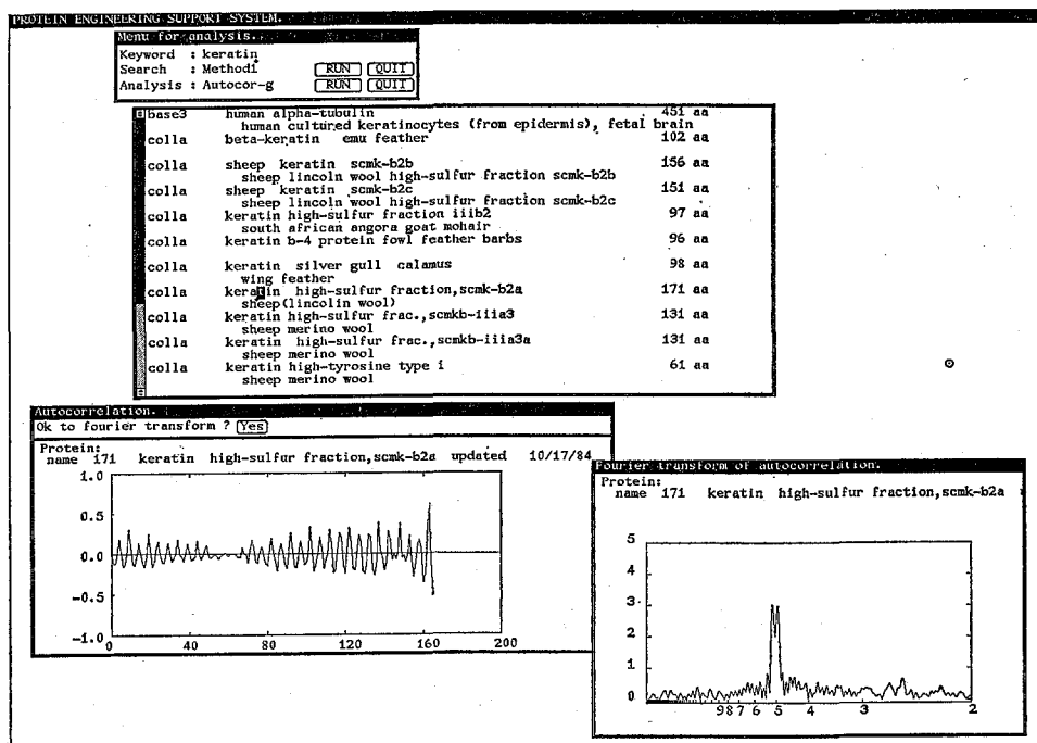
Fig. 3. The periodic pattern in the sequence of sheep keratin B2A calculated by the autocorrelation function \overline{A(\tau)} and its Fourier transform.
