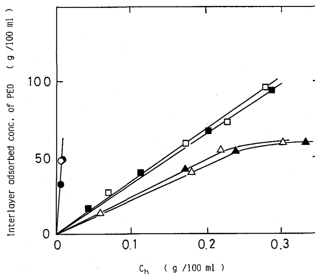
Figure 6. Initial slope of isotherms for the adsorption of PEO 400 at 35°C, \Delta and at 15°C, \blacktriangle ; PEO 6,000 at 35°C, \square and \blacksquare at 15°C; PEO 20,000 at 35°C, \circ and at 15°C, \bullet on Ca montmorillonite.
