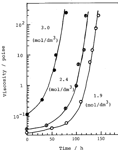
Fig. 3. Viscosity change as a function of aging time for sol 1( \text{Al}_2\text{O}_3 , 3.0), sol 2( \text{Al}_2\text{O}_3 , 2.4) and sol 3( \text{Al}_2\text{O}_3 , 1.9 mol/dm 3 ), respectively.
