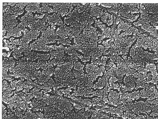
Fig. 2. Scanning electron micrographs of 3.0 nm Au films evaporated on (A) 1-monolayer and (B) 7-monolayers stearic acid LB films on Ge plate. Many straight lines in (A) are scratches on the Ge surface.
