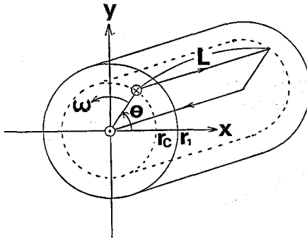
Fig. 4. Scheme of sense coil.
