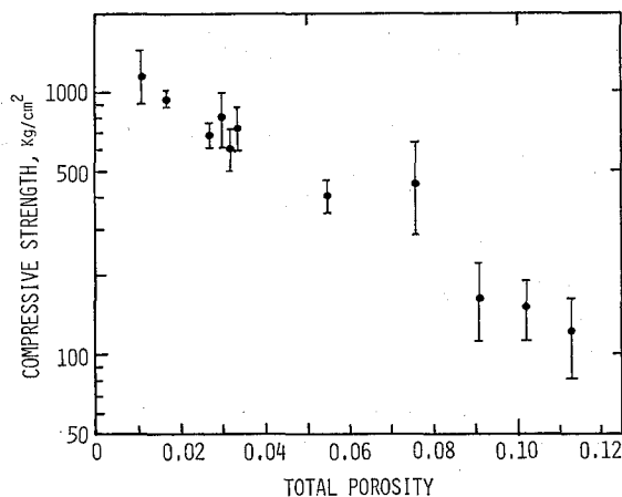
Fig. 16. Compressive strengths of the ingots in the direction perpendicular to their solidification directions as a function of their porosities.
