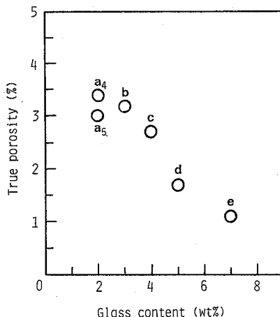
Fig. 12. True porosities of the cylindrical-pore-free ingots versus their glass contents.
