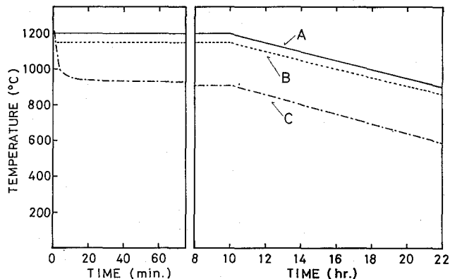
Fig. 2. Temperature changes at the top of the crucible (A), the upper surface of the melt (B) and the inner surface of the bottom of the crucible (C) during solidification process in which the temperature at the top of the crucible was first maintained at 1200°C for 10 h and then lowered at a rate of 25°C/h.
