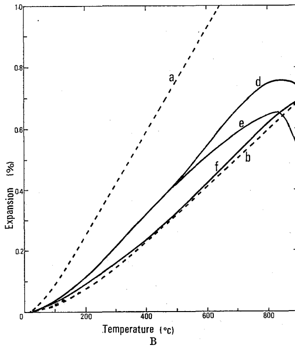
Fig. 14. Thermal expansions of the \text{Li}_2\text{O}\cdot 2\text{SiO}_2 (d), 100(\text{Li}_2\text{O}\cdot 2\text{SiO}_2)3\text{Na}_2\text{O} (e) and 100(\text{Li}_2\text{O}\cdot 2\text{SiO}_2)3\text{Al}_2\text{O}_3 (f) ingots all solidified at a rate of 1.3 mm/h, in the directions parallel (A) and perpendicular (B) to the solidification direction, respectively. a, b, and c; Thermal expansions of \text{Li}_2\text{O}\cdot 2\text{SiO}_2 single crystal in its a-, b- and c-axes.
