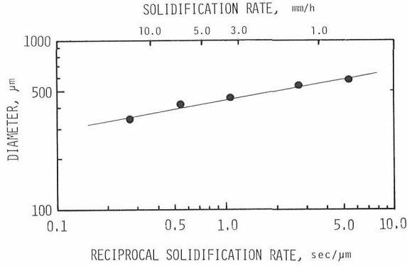
Fig. 6. Mean diameter of the Li 2 O·2SiO 2 columnar crystals in the ingots as a function of their solidification rates.
