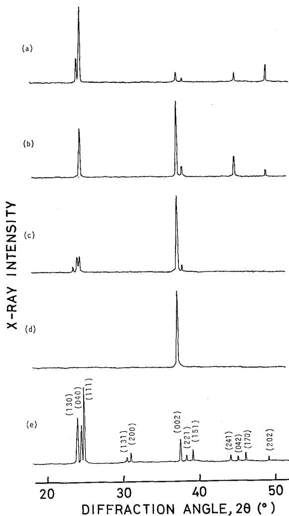
Fig. 4. The X-ray diffraction patterns taken of the transverse sections of the Li 2 O·2SiO 2 ingots solidified in various clay crucibles the bottom surface of which had been fresh (a), or covered with a platinum foil (b), a sintered Li 2 O·2SiO 2 ceramic plate (c) or a Li 2 O·2SiO 2 glass-ceramic layer (d). The pattern (e) is that of powdered Li 2 O·2SiO 2 crystals.
