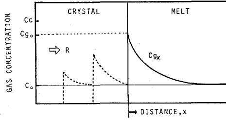
Fig. 9. Schematic representation of gas distribution in a solidifying melt.
