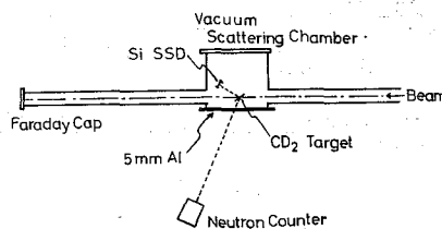
Fig. 5. Experimental setup for efficiency determination.
