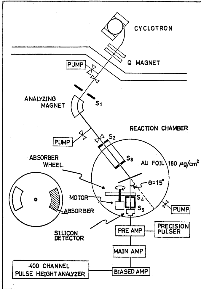
Fig. 1 Experimental setup for the energy loss measurement.
