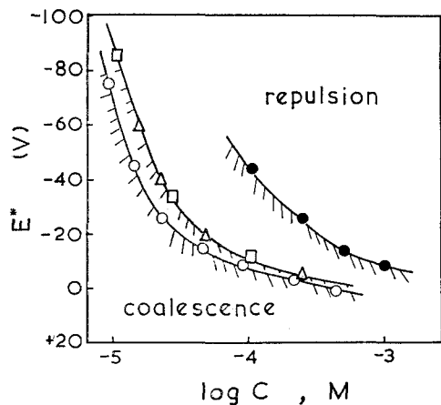
Fig. 2. The influence of the surface active agent concentration on the coalescence of the aqueous droplet in the oil phase. Aqueous phase: 0.1 M KCl. Oil phase: ●, DPC; △, CPC; □, CTAC; ○, OTAB.
