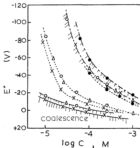
Fig. 3. The influence of the composition of the aqueous and oil phases on the coalescence of the aqueous droplet. Aqueous phase: ---, 0.1 M KBr; ....., 0.1 M KCl; ——, 0.1 M KF. Oil phase: ●, DPC; △, CPC; ○, CTAC; ×, OTAB.
