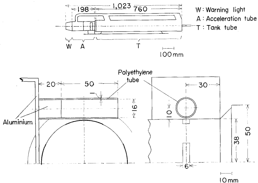
Fig. 1. Schematic diagram of the activation geometry.
