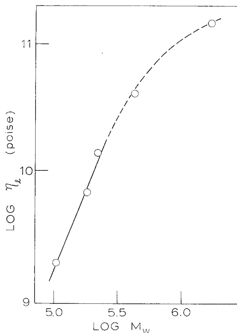
Fig. 7 \eta_s at 200° plotted logarithmically against M_w for five poly- \alpha -methylstyrene samples.
