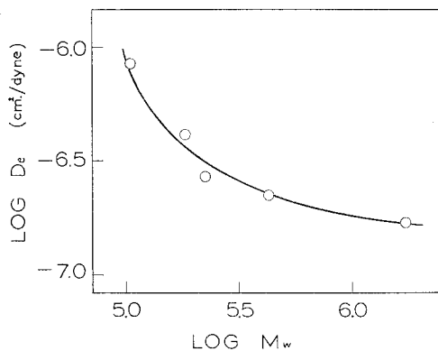
Fig. 6 D_e at 200° plotted logarithmically against M_w for five poly- \alpha -methylstyrene samples.
