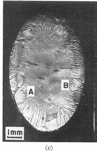
Fig. 3. (a) Macro-structure of the side surface, (100), of a 99.99% lead crystal grown at the lowering rate of 41 mm/min. (b) Enlarged photograph of a part of (a). (c) Optical micrograph of the transversal section, (00 \bar{1} ), at the part shown with an arrow in (a).
