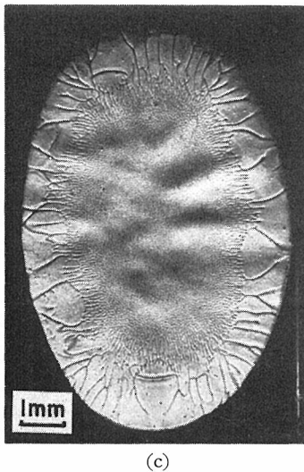
Fig. 2. (a) Macro-structure of the side surface, (100), of a 99.99% lead crystal grown at the lowering rate of 23 mm/min. (b) Enlarged photograph of a part of (a). (c) Optical micrograph of the transversal section, (00 \bar{1} ), at the part shown with an arrow in (a).
