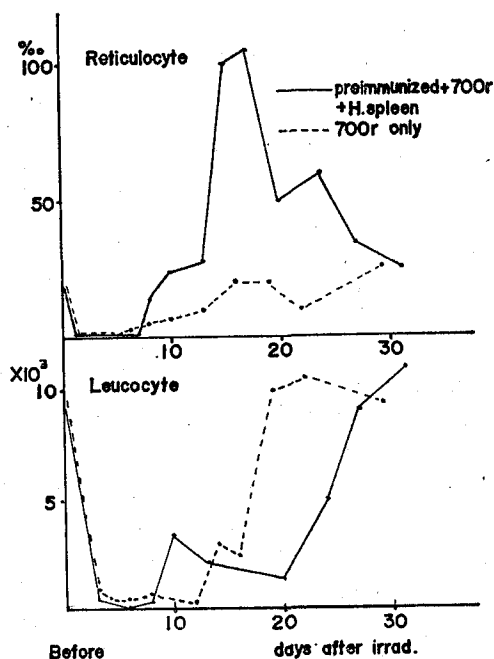
Fig. 2. Changes of leucocyte and reticulocyte count.
