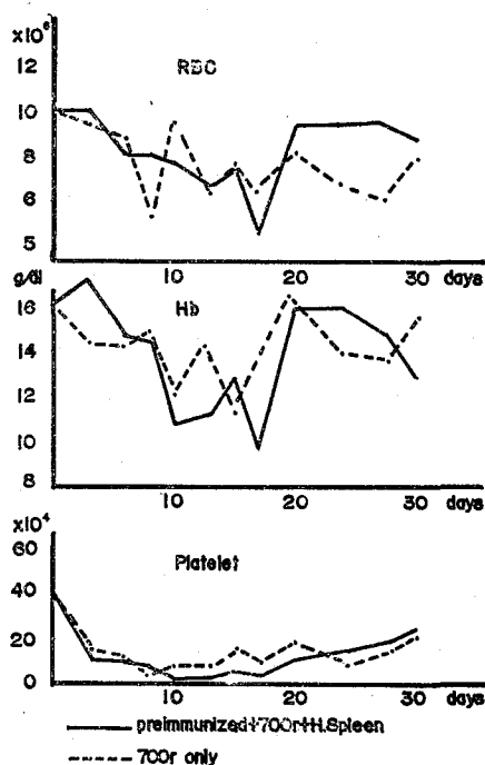
Fig. 1. Changes of RBC, Hb and platelet count.
