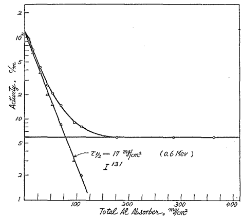
Fig. 13 : \beta -ray Absorption Curve, I^{131} : Applied potential ; 1350 V, Geometry ; sample 3rd shelf, absorber 2nd shelf
