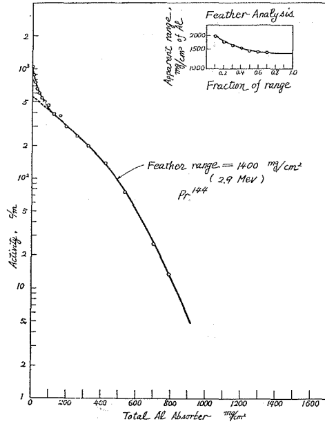
Fig. 11 : \beta -ray Absorption Curve, Ce^{144}-Pr^{144} : Applied potential ; 1350 V, Geometry ; sample 3rd shelf, absorber 2nd shelf
