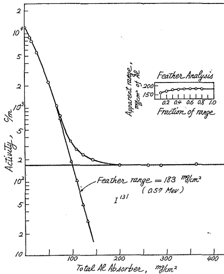
Fig. 5 : \beta -ray Absorption Curve, I (original sample) : Applied potential ; 1350 V, Geometry ; sample 3rd shelf, absorber 2nd shelf.
