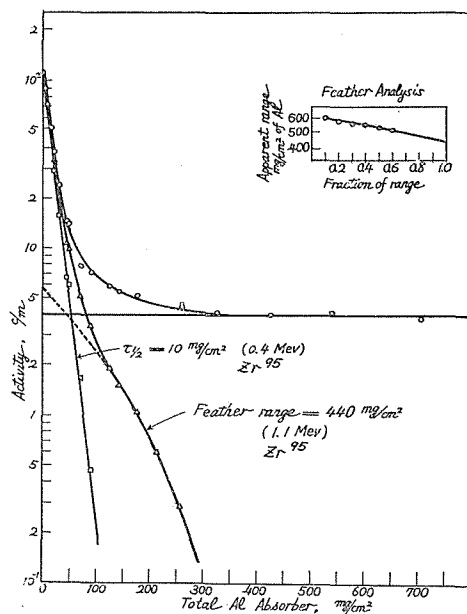
Fig. 23 : \beta -ray Absorption Curve, Zr 95 - Nb 95 : Applied potential ; 1350 V, Geo- metry ; sample 3rd shelf, absorber 2nd shelf.
