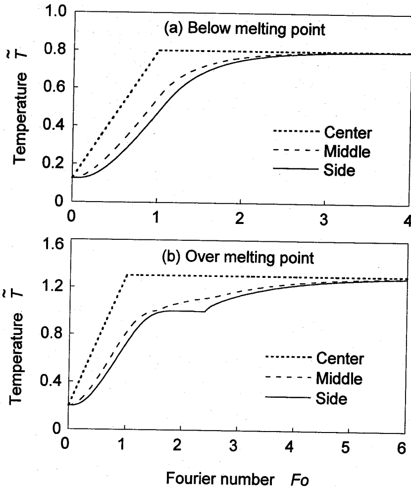
Fig.6.2. Numerical solution of heat conduction equation.
