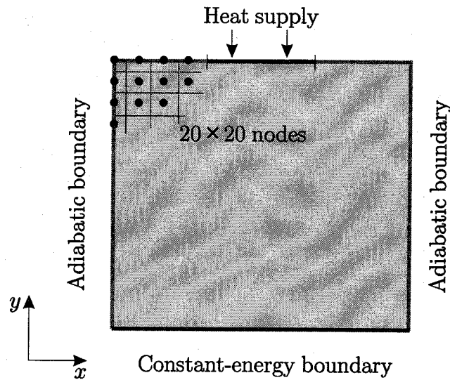
Fig.7.21. Two-dimensional FDM model for melting/solidification simulation by energy conduction equation.
