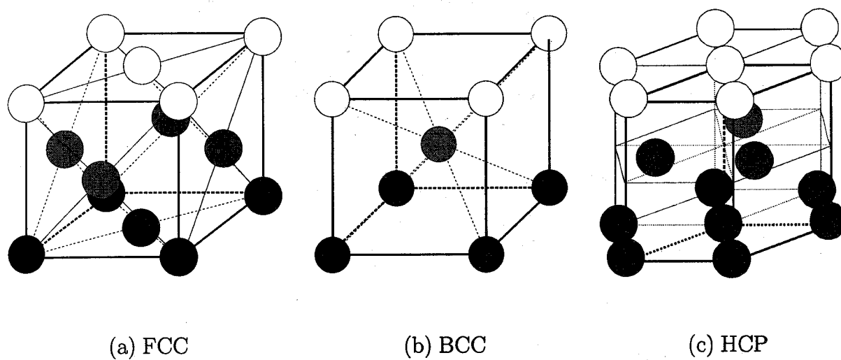
Fig.5.1. Crystallographical view of fcc, bcc and hcp structure.
