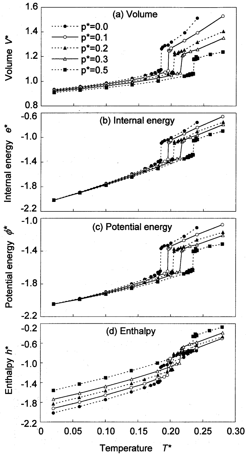
Fig.3.6. Temperature dependence of volume, internal energy, potential energy and enthalpy with isobaric lines.
