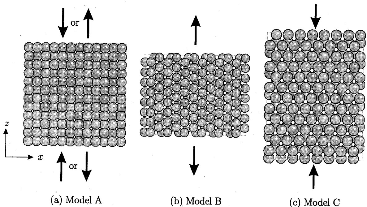
Fig.5.7. Simulation models applied in compression and tension of fcc and hcp.
