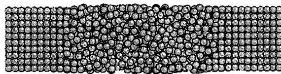
(a) 15000 step
