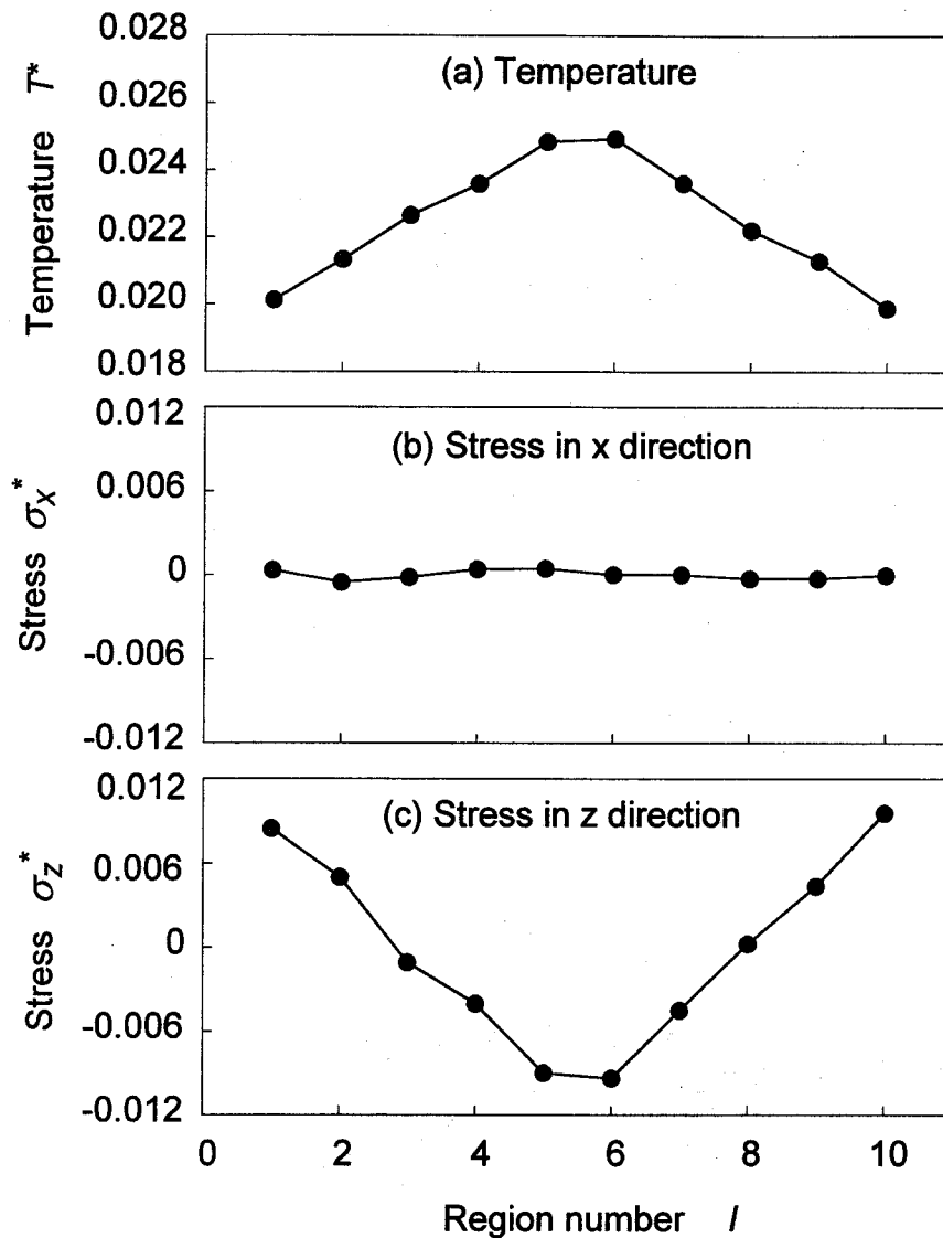
Fig.4.6. Temperature gradient and thermal stress in each region.
