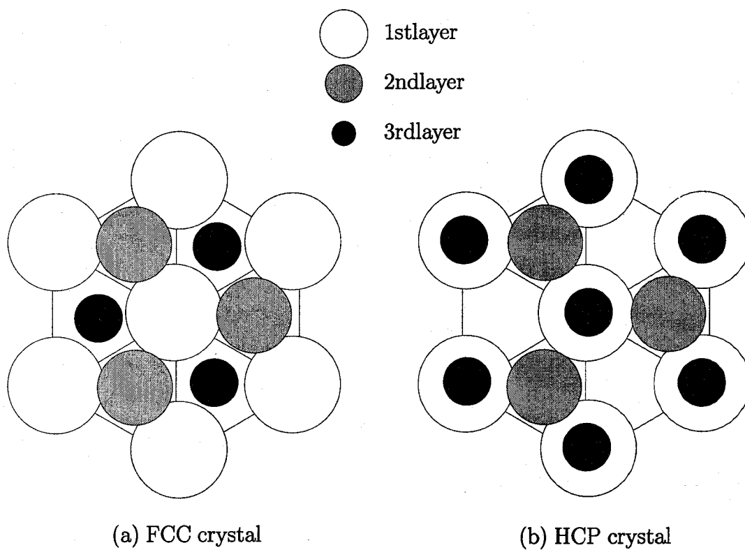
Fig.5.2. Layer order of closed-packed plane of fcc and hcp.
