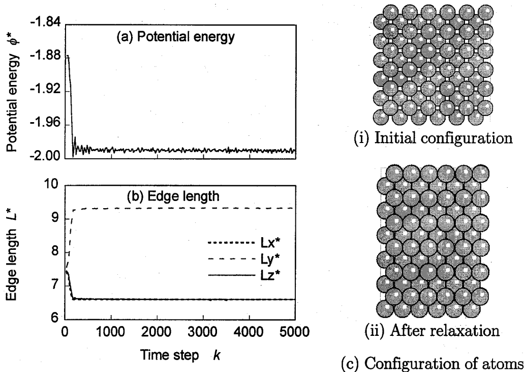
Fig.5.6. Variation of potential energy and edge lengths and change in the configuration of atoms initiated by bcc crystal.
