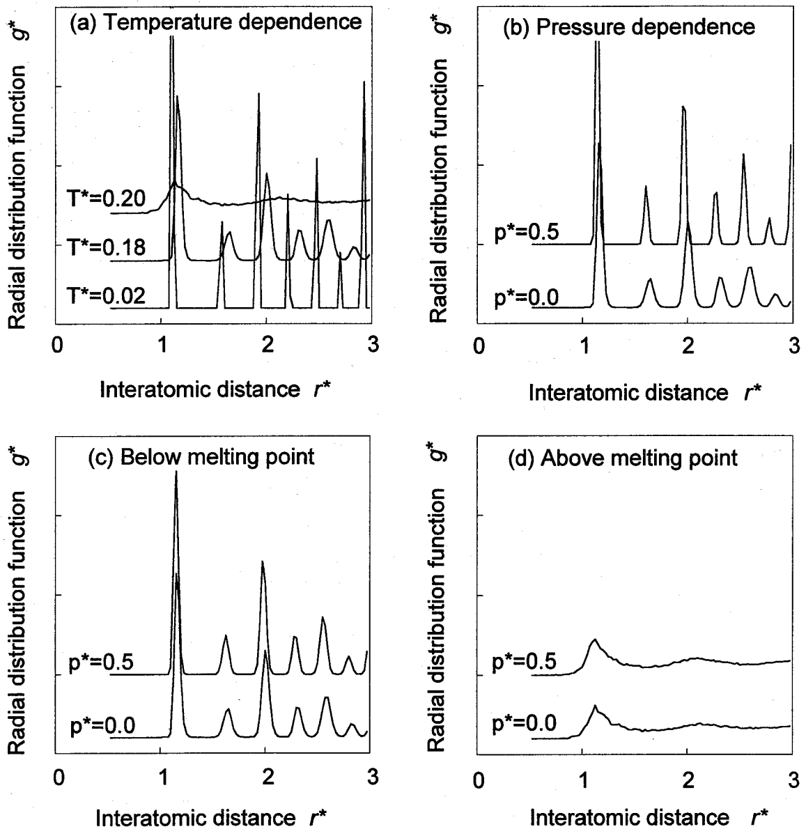
Fig.3.8. Radial distribution functions under various conditions of temperature and pressure.
