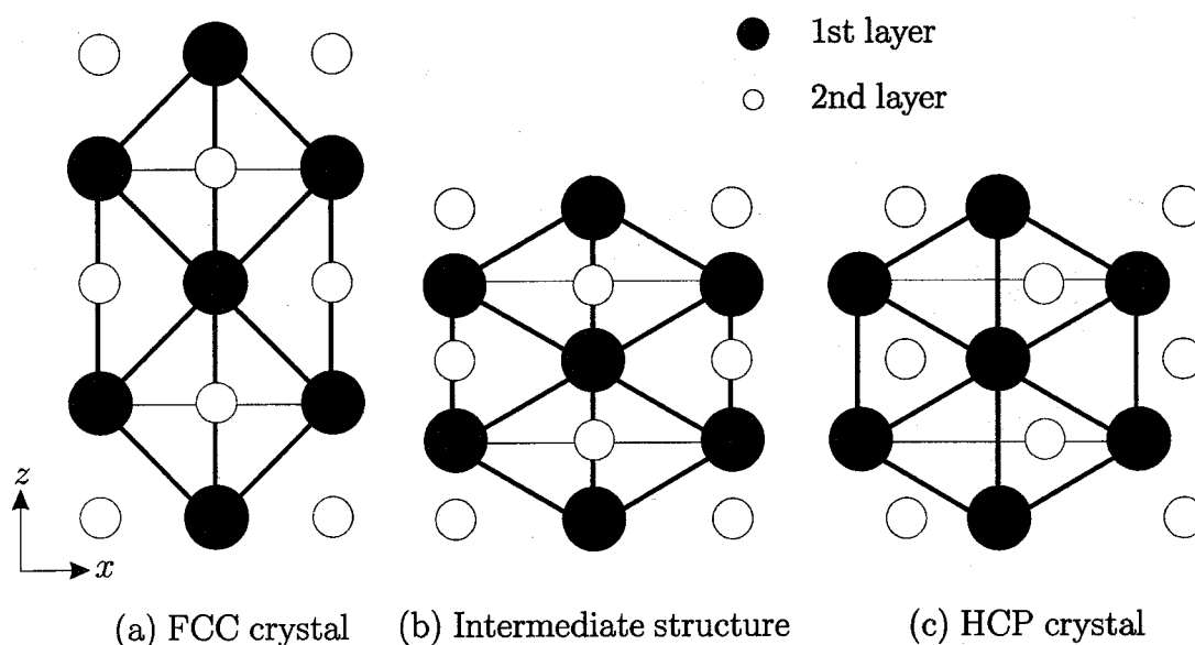
Fig.5.4. Crystallographical relation between fcc and hcp structure.
