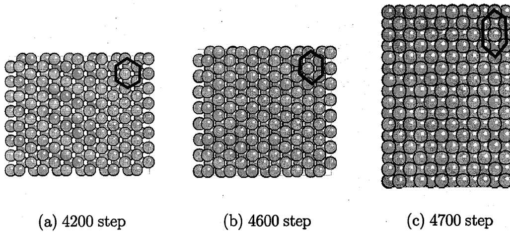
Fig.5.25. Structural change during stress-controlled tension of hcp.
