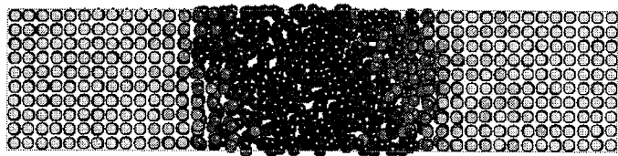
(c) 15000 step
