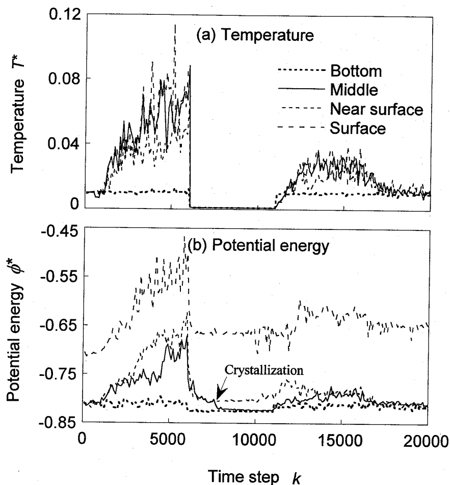
Fig.7.18. Variation of temperature and potential energy during successive heating and cooling processes.
