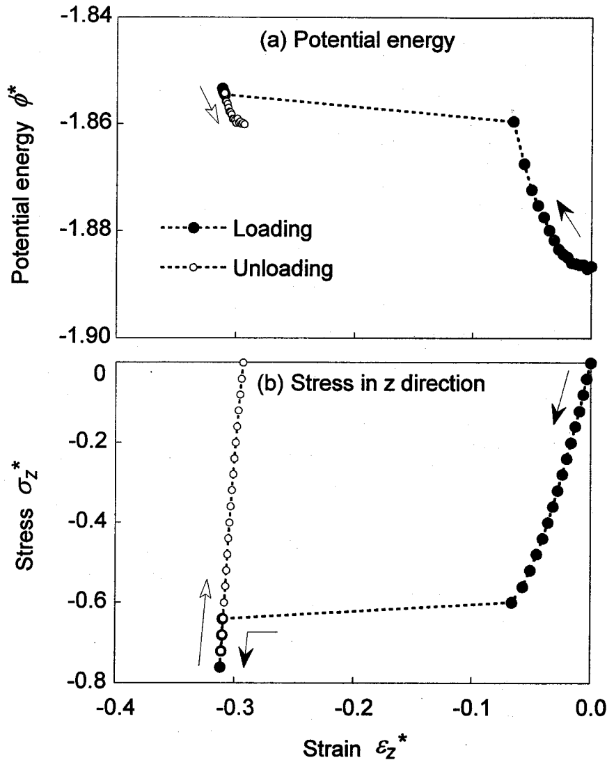
Fig.5.21. Potential energy and stress plotted against strain during loading and unloading.
