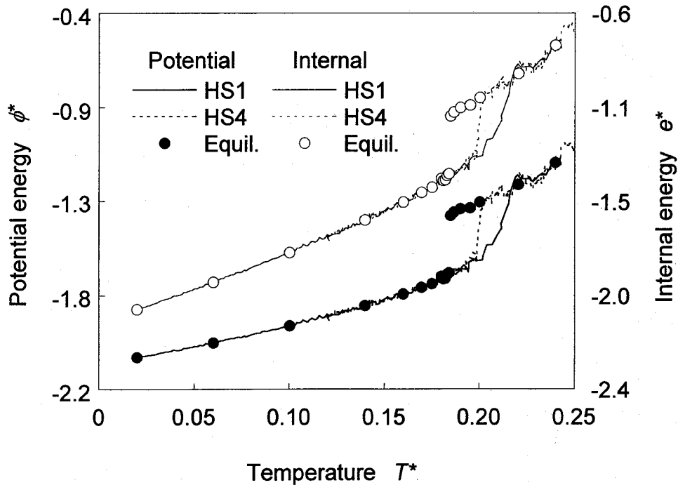
Fig.3.14. Relation between internal and potential energy and temperature during heating by velocity scaling method under conditions HS1 and HS4, compared with that of equilibrium state.
