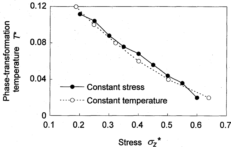
Fig.5.41. Dependence of threshold temperature on stress.
