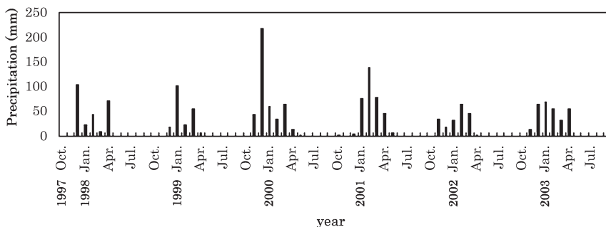
Fig. 7. Precipitation in Onkani village (1997–2003).
