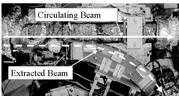
Figure 4. The magnetic septum. After the deflection of the ESS, septum thickness of 22.6 mm is provided for the septum magnet. With the field of 0.5T and the pole length of 550 mm the extracted beam is deflected as large as 45° and is guided to the extraction beam line.
