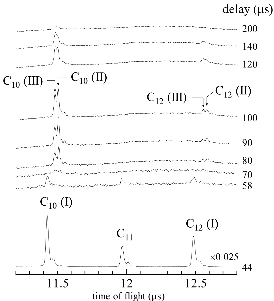
Fig. 3-9 TOF mass spectra of laser ablation of graphite in heated He gas observed by one-photon ionization. The temperature of the buffer gas at the exit was about 600 K. Only the spectral region of \text{C}_{10} , \text{C}_{11} and \text{C}_{12} is shown. The numbers to the right of the spectra represent the delay times in \mu\text{s} of the ionization laser pulse relative to the ablation pulse. The spectrum observed at the delay time of 35 \mu\text{s} is multiplied by a factor of 0.025.
