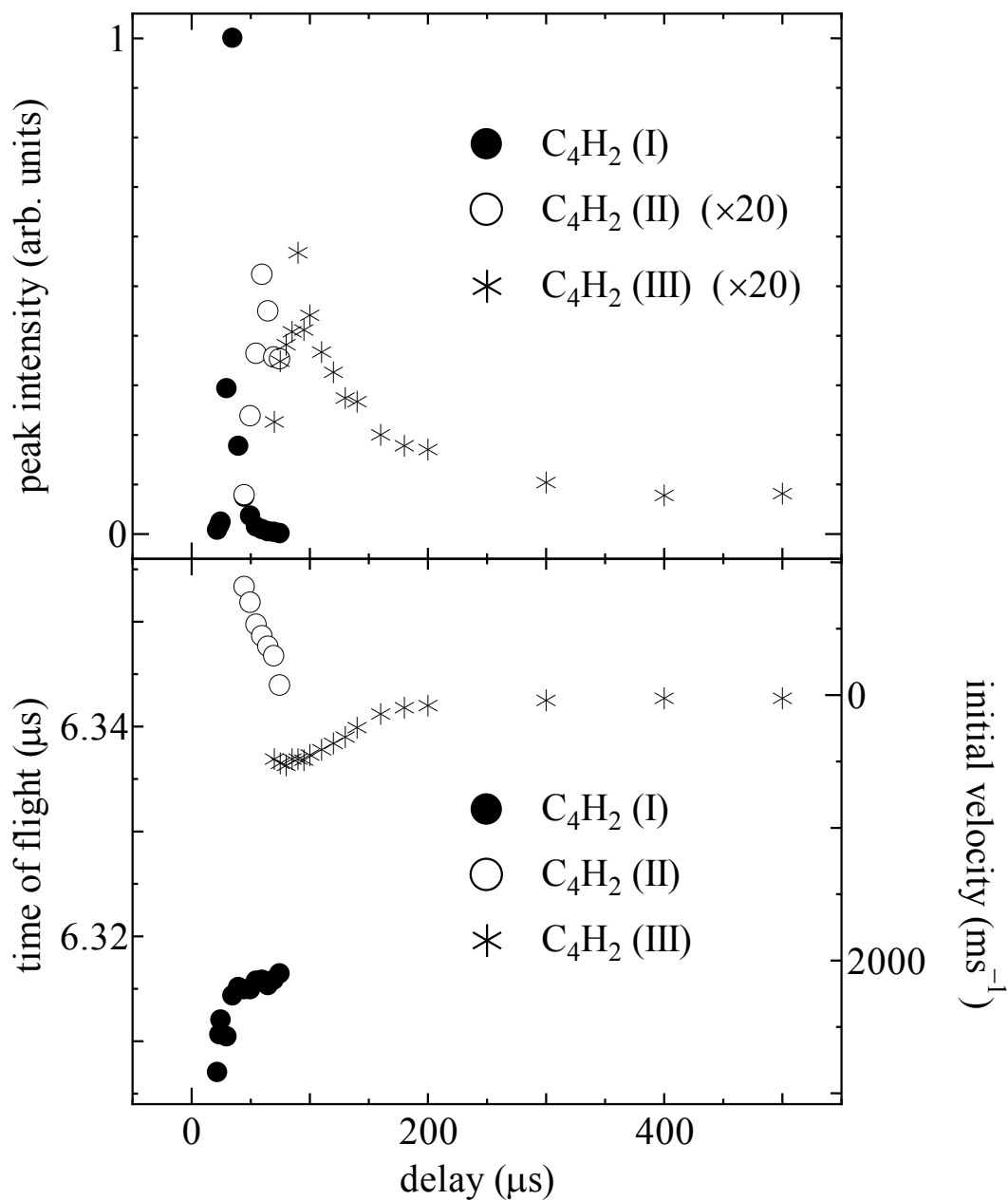
Fig. 3-4 Change of peak intensity (top) and shift of TOF (bottom) of \text{C}_4\text{H}_2 as a function of the delay time of ionization pulse relative to the ablation pulse. Signals corresponding to the first (I), second (II), and third (III) components are displayed as closed circles ( \bullet ), open circles ( \circ ) and asterisks ( * ), respectively. The peak intensities of the second and third components are multiplied by a factor of 20.
