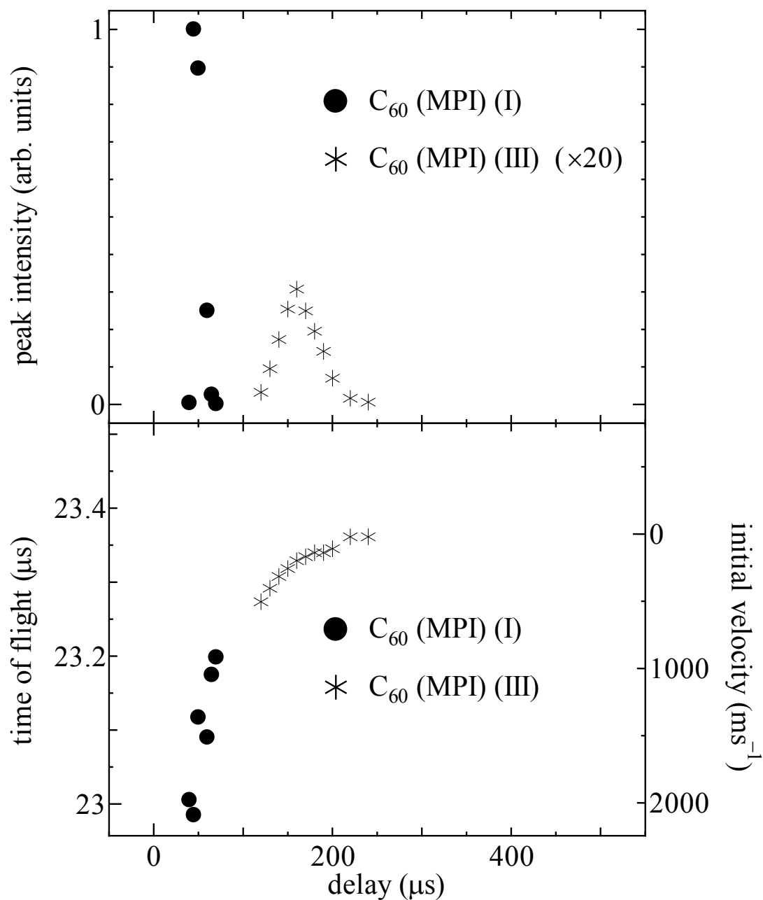
Fig. 3-13 Change of peak intensity (top) and shift of TOF (bottom) of \text{C}_{60} observed in He buffer gas with MPI. Signals corresponding to the first (I) and third (III) components are displayed as closed circles ( \bullet ) and asterisks ( * ) respectively. The peak intensities of the third component are multiplied by a factor of 20.
