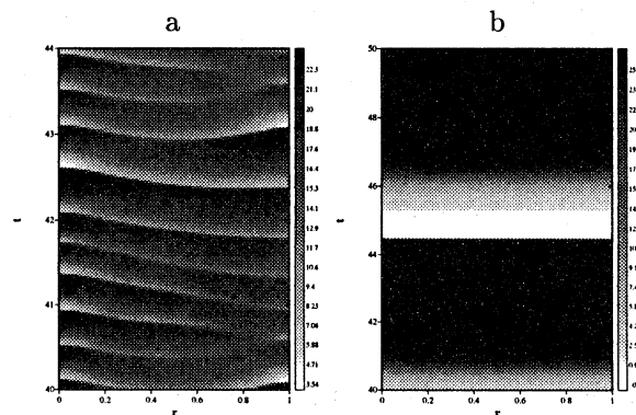
Figure 4: Spatio-temporal evolution of the potential for the hallow cylinder configuration, (a) V = 26.55 and (b) V = 27.76 .
