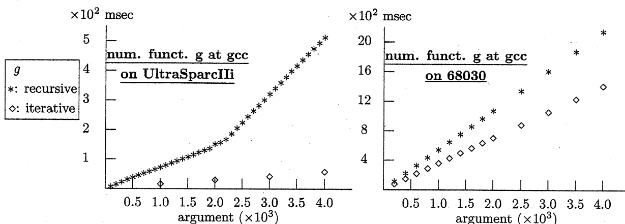
Figure 3: Results of numeric function g at gcc: on UltraSparcIII (left) and on 68030 (right)
