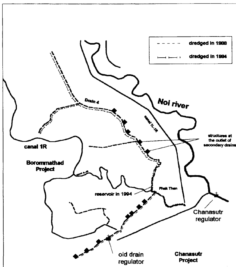
Fig. 7 Drainage Improvements
