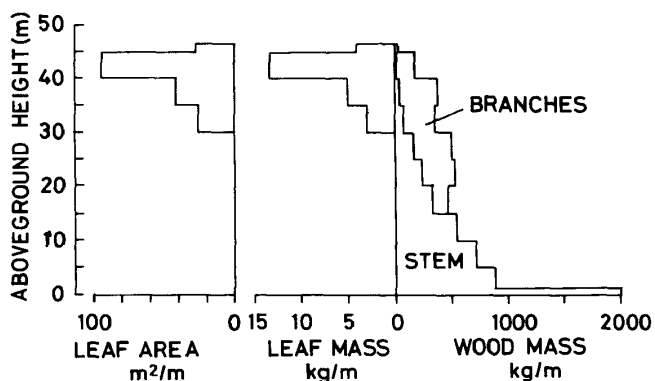
Fig. 5 Plant mass profile of a large canopy tree, Dipterocarpus crinitus
