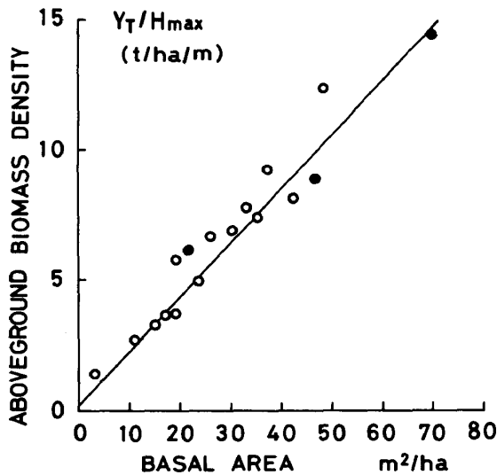
Fig. 10 Linear relation between basal area and aboveground biomass density defined by the ratio of aboveground biomass ( Y_T ) to the maximum tree height ( H_{max} ) in the stand. Open circles and closed circles represent observed values. The mark's differences result from the lower limit of DBH in the computation of basal area (○, DBH \geq 4.5 cm; ●, DBH \geq 10 cm). The straight line represents calculated values of Eqn (2).
