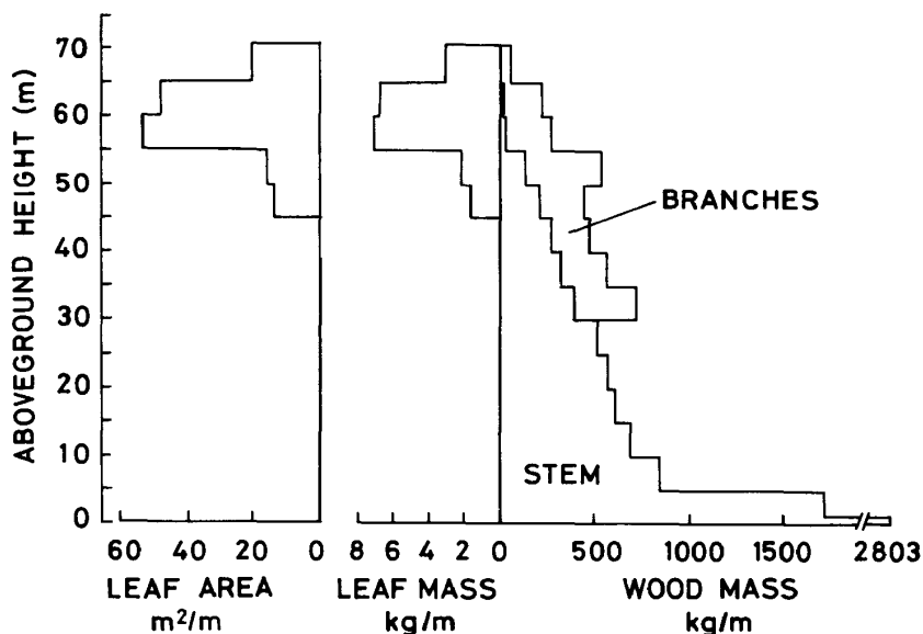
Fig. 3 Vertical changes of leaf area, leaf mass, and wood mass at different horizontal strata of an emergent tree, Shorea laevis
