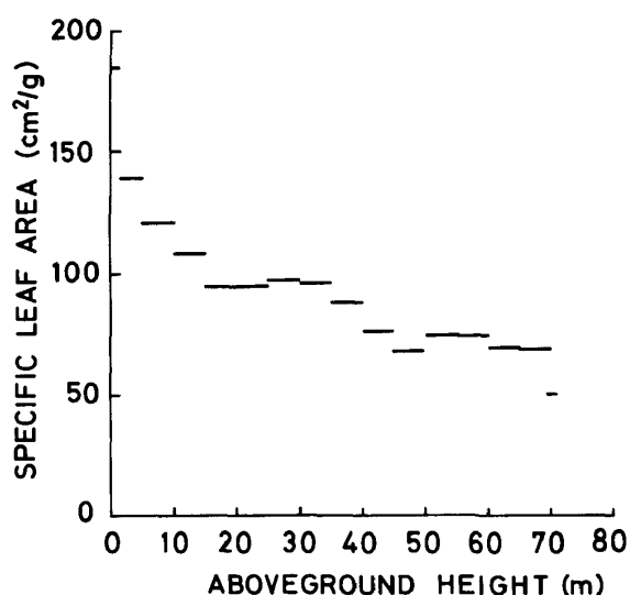
Fig. 9 Decrease of specific leaf area with an increase of aboveground height
