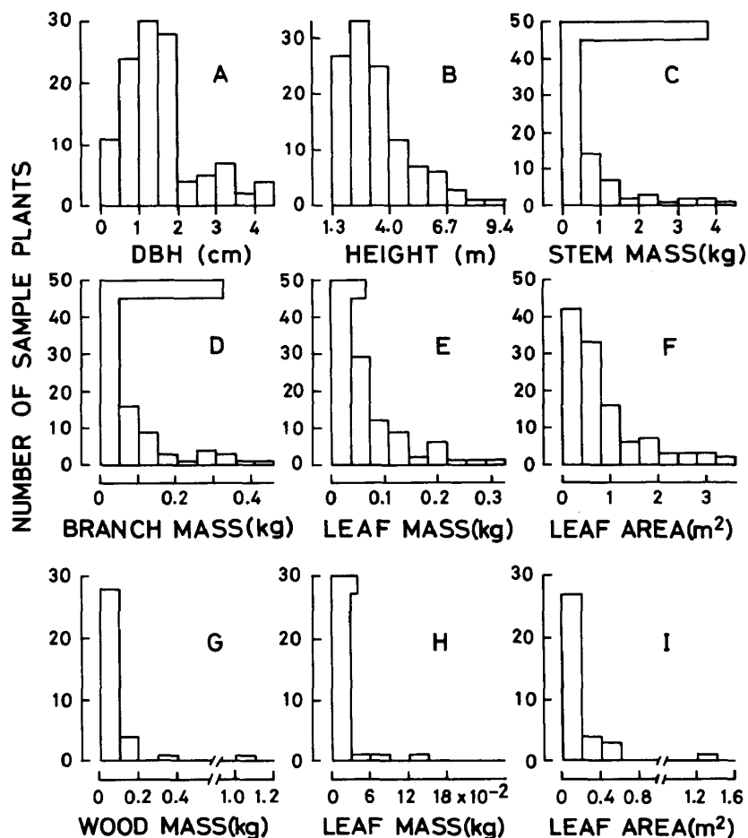
Fig. 7 Frequency distribution of various measurements of small plants (DBH < 4.5 cm and tree height \geq 1.3 m) sampled from four 5 m \times 5 m quadrats. Six figures, Figs. 7A–7F, represent independent plants and the other figures, Figs. 7G–7I, represent the samples of dependent plants supported by independent plants.
