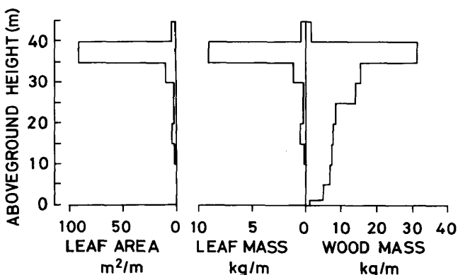
Fig. 6 Vertical distribution of various plant masses of dependent plants living on the large Dipterocarpus crinitus
