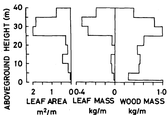
Fig. 4 Vertical distribution of leaf area, leaf mass, and wood mass of dependent plants supported by the emergent Shorea laevis
