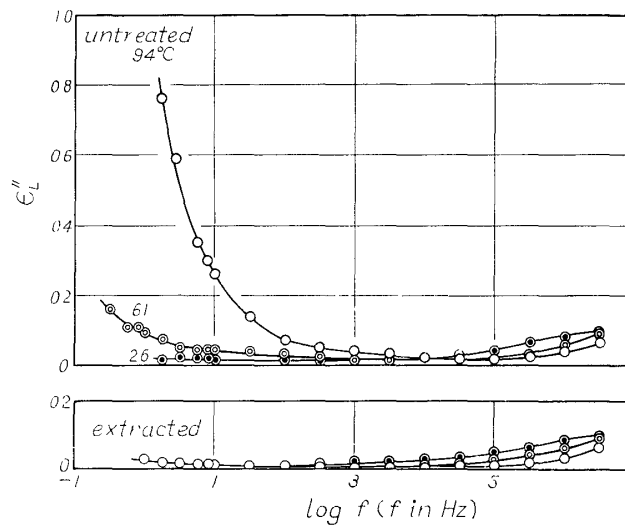
Fig. 8. The dielectric loss factor of the untreated and the extracted oven dried HINOKI at 26, 61 and 94°C.
