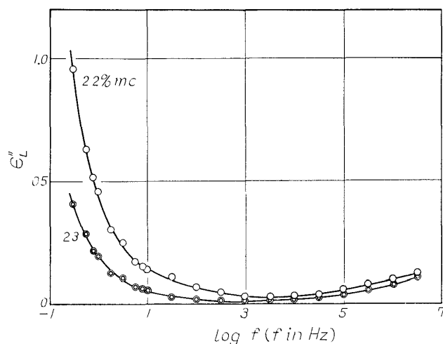
Fig. 9. The dielectric loss factor of the untreated and the extracted HINOKI at 2.2-2.3 % m. c. as a function of frequency. ○ : the untreated, ● the extracted
