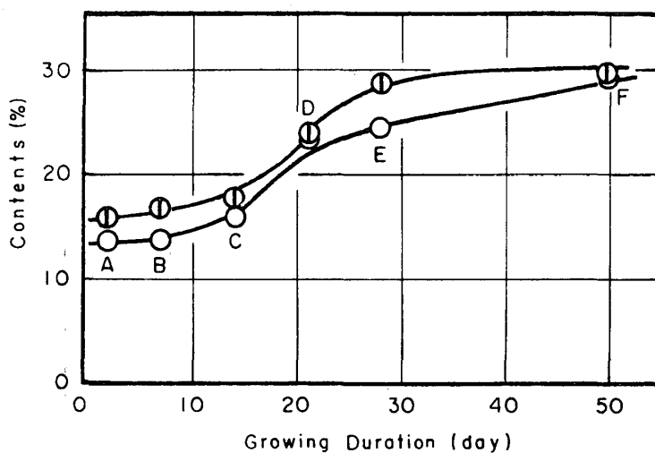
Fig. 4. The changes of \alpha -cellulose and lignin contents of hypocotyls with growing duration. \odot and \circ indicate \alpha -cellulose and lignin contents respectively. A, B, C, D, E and F correspond to the samples as illustrated in Fig. 1.
