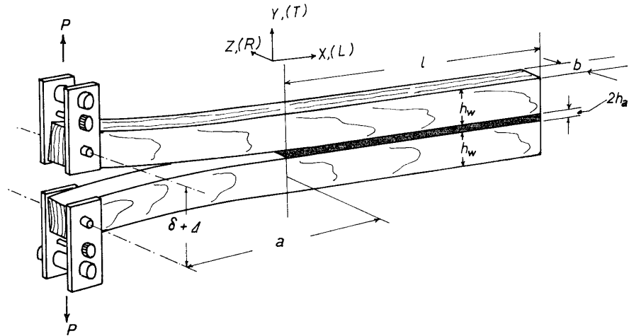
Fig. 1. Double Cantilever Beam (DCB) specimen with thick adhesive alyer. a: crack (beam) length, l: glue line length, h_w : depth of beam, b: thickness of specimen, 2h_a : thickness of glue line, \Delta=2h_a+h_w , P: load, \delta : deflection.
