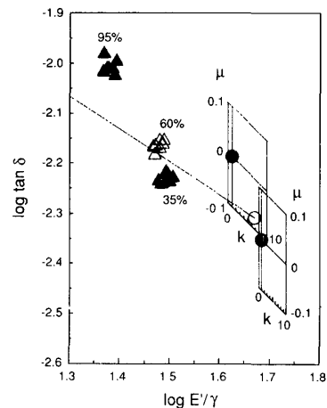
Fig. 2. Effect of water in the cell wall on the \log E'/\gamma - \log \tan \delta relationship. The broken line shows the experimental correlation for untreated specimens. Various values of relative increase of matrix rigidity ( k ) and mobility factor ( \mu = \log(k/s) ) were simulated. \triangle , \blacktriangle : experimental values; \circ , \bullet : theoretical plot for zero MMA.
