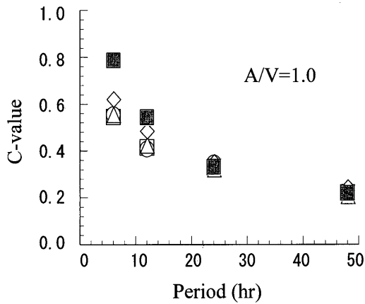
Fig. 2. The change in C value for sugi wood with period measured at A/V=1 at different temperature amplitude. Temperature amplitude: 2.5^{\circ}\text{C} ( \square ), 5^{\circ}\text{C} ( \circ ), 7.5^{\circ}\text{C} ( \triangle ), 10^{\circ}\text{C} ( \diamond ). Calculated value ( \blacksquare ).
