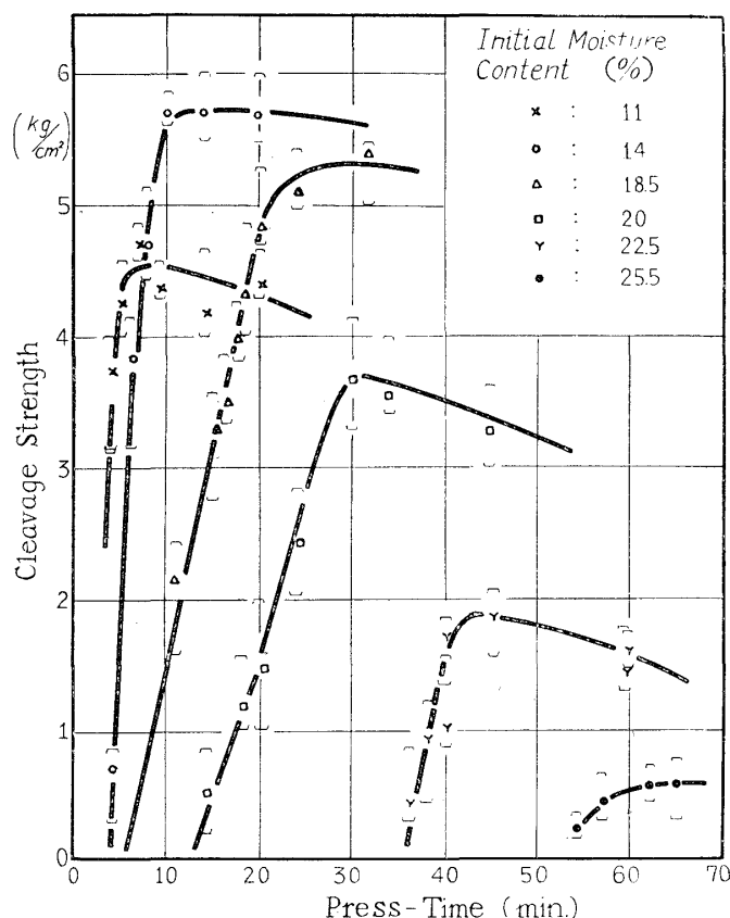
Fig. 3. Relation between cleavage strength and press-time. (G-type, spec. gravity 0.65, board thickness 20 mm)
