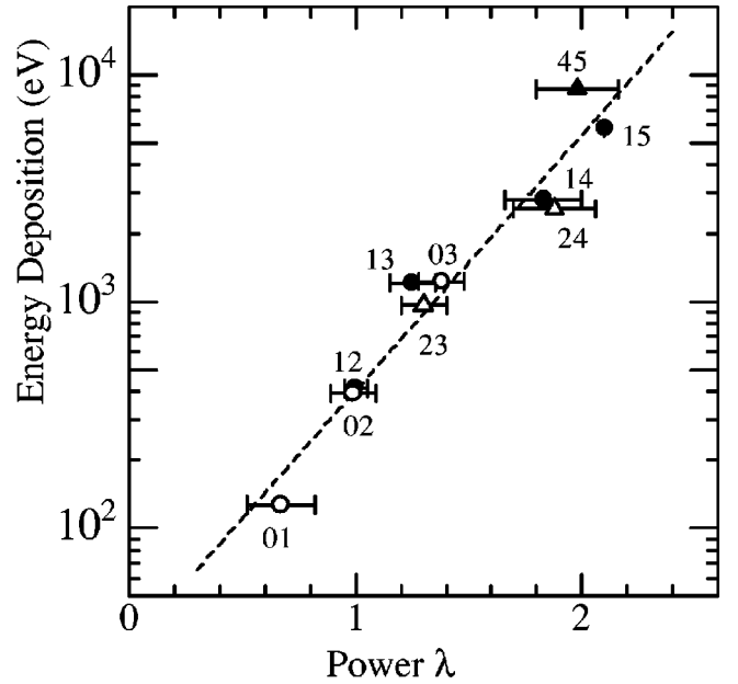
FIG. 8. Calculated energy deposition E_{qk} for q \rightarrow k loss collisions as a function of the experimentally determined power \lambda . The dashed line is the fitting result; E(\lambda) = 30 \exp(2.6\lambda) .
