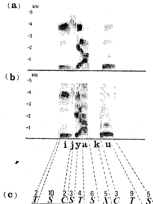
Fig. 3. Synthesized speech [ijaku] (胃弱) (a) sonogram of natural input speech (b) sonogram of synthesized speech (c) result of segmentation
