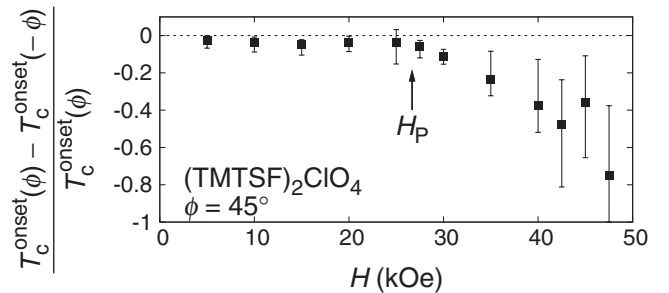
FIG. 4. Field dependence of the relative difference between T_c^{\text{onset}}(+45^\circ) and T_c^{\text{onset}}(-45^\circ) .
