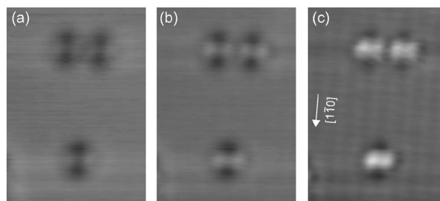
FIG. 2. Typical STM images of three monomers ( C_2H_2 ) obtained at (a) V_s=-0.25 \text{ V} , (b) V_s=-0.1 \text{ V} , and (c) V_s=-7 \text{ mV} with I_t=0.5 \text{ nA} ( 32 \times 45 \text{ \AA}^2 ). An elongated protrusion appears in (c) with a faint dent in the center, which reflects the nodal plane of the out-of-plane \pi^* orbital of the molecule. The atomic rows are simultaneously observed in (c), indicating that acetylene molecule adsorbs in the trough of Cu(110).
