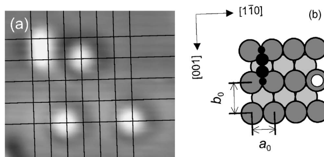
FIG. 3. (a) A STM image of acetylene ( C_2H_2 ) coadsorbed with carbon monoxide (CO) at V_s=-0.15 \text{ V} and I_t=5 \text{ nA} ( 23 \times 29 \text{ \AA}^2 ). The former appears as an elongated protrusion along the [001] direction, while the latter shows round protrusion. CO molecules adsorb at the on-top site and the grid lines are depicted through Cu atoms of the substrate. The adsorption site of acetylene is thus determined to be fourfold hollow site, as schematically shown in (b). The black and white circles indicate acetylene and CO molecules, respectively.
