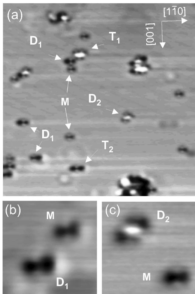
FIG. 1. A typical STM image of Cu(110) exposed to acetylene ( C_2H_2 ) at 40 K. (a) A large-scale image ( 280 \times 280 \text{ \AA}^2 ) showing isolated monomer ( M ), and a variety of clusters such as dimers ( D_1, D_2 ), trimers ( T_1, T_2 ), and larger islands. V_s=0.1 \text{ V} , I_t=0.1 \text{ nA} . Two types of dimer are shown in (b) and (c) in comparison with a monomer ( 29.5 \times 29.5 \text{ \AA}^2 ). (b) The dimer ( D_1 ) appears as an asymmetric dark dumbbell composed of two molecules adjoined along the [1\bar{1}0] direction. V_s=-0.1 \text{ V} , I_t=0.2 \text{ nA} . (c) The dimer ( D_2 ) consists of two monomers adjoined along the low-symmetry direction with a pronounced protrusion in between. V_s=-0.1 \text{ V} , I_t=0.2 \text{ nA} .
