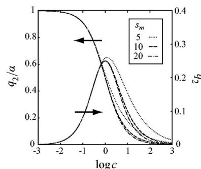
FIG. 9. The probability for a randomly selected associated group to be in a pairwise junction (left), and the fraction of functional groups belonging to pairwise junctions (right) plotted against the reduced polymer concentration. The maximum multiplicity of the junctions is varying from curve to curve.
