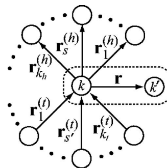
FIG. 14. The number of the states described in this figure is given by Eq. (A2). Circles stand for junctions and arrows linking two junctions represent the head-to-tail vector of the chain (chains are not shown here for simplicity).
