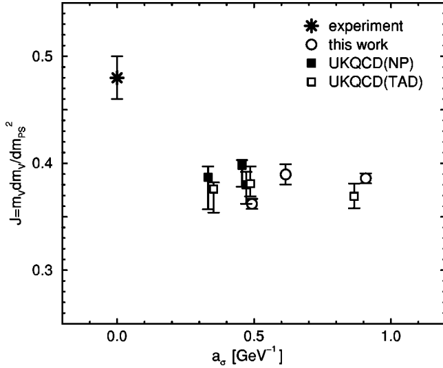
FIG. 11. The parameter J . The a_\sigma is set by using r_0 . Data from UKQCD Collaboration (square symbols) are taken from Ref. [15] on isotropic lattices, and slightly horizontally shifted.
