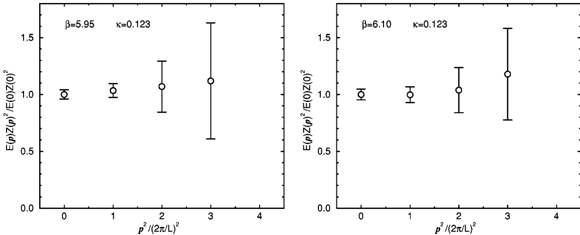
FIG. 12. The covariance of the pseudoscalar correlators. The left panel is at \beta = 5.95 and \kappa = 0.1230 , and the right at \beta = 6.10 and \kappa = 0.1230 .
