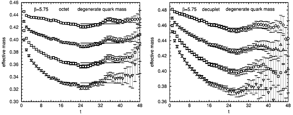
FIG. 9. Effective mass plots for octet and decuplet baryon correlators with degenerate quark masses at \beta=5.75 . Horizontal solid line represent the fit range and the mass from the single exponential fit.
