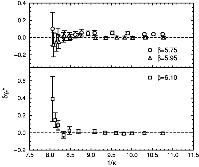
FIG. 6. \delta\gamma_F^* = \gamma_F^{*(PS)} - \gamma_F^{*(V)} at \beta=5.75 and 5.95 in the upper part and 6.10 in the lower part.
