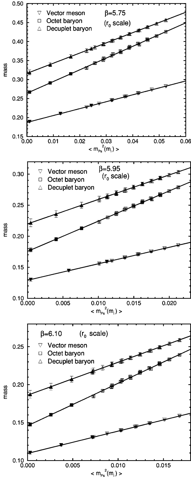
FIG. 10. The masses of vector mesons and octet and decuplet baryons together with the result of linear fits. Only the \Sigma -type octet baryon is shown. The filled symbols correspond to the masses at the physical u , d , and s quark masses with the scale set by r_0 .
