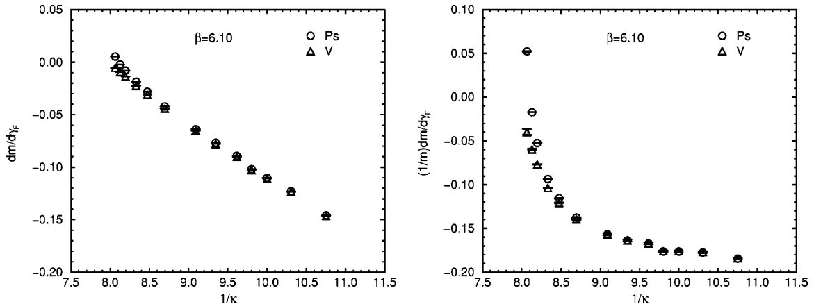
FIG. 8. The response of meson masses to a change of \gamma_F at \beta=6.10 . The left panel shows dm/d\gamma_F , while the ratio (1/m)dm/d\gamma_F is shown on the right. The results for the pseudoscalar and vector mesons are represented by circles and triangles, respectively.
