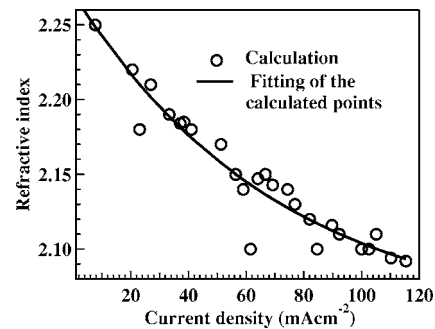
FIG. 4. Refractive index estimated from the FFT peak position as a function of current density. The optical thickness can be estimated as half of the peak position.
