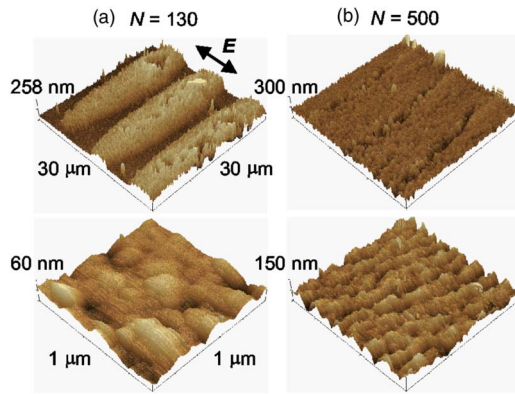
FIG. 2. (Color online) SPM images of the DLC surfaces irradiated with (a) N=130 and (b) N=500 at F=0.14 \text{ J/cm}^2 and \Delta t=0 with the parallel polarizations. The upper image is for the central area of 30 \times 30 \mu\text{m}^2 and the lower is for 1 \times 1 \mu\text{m}^2 on the focal spot. The polarization direction is denoted with the arrows.
