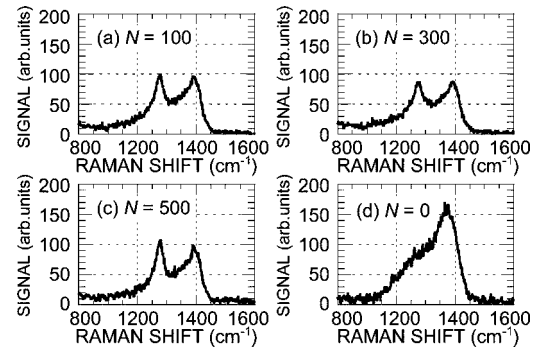
FIG. 3. Raman spectra of DLC surfaces irradiated with (a) N=100 , (b) N=300 , and (c) N=500 at F=0.14 \text{ J/cm}^2 , together with (d) the spectrum of nonirradiated DLC. The experimental conditions for (a), (b), and (c) are the same as those at (A), (B), and (C) in Fig. 1(b).
