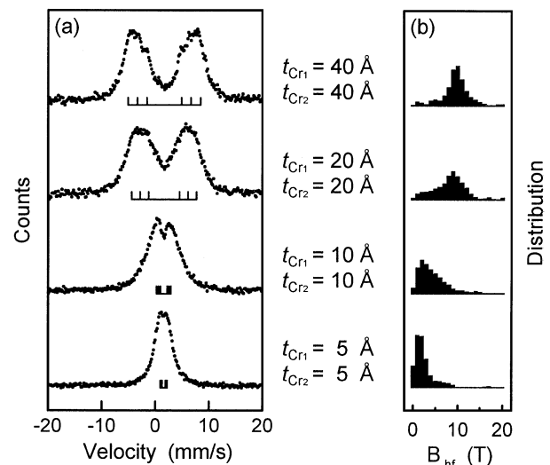
FIG. 2. (a) ^{119}\text{Sn} Mössbauer spectra for [Fe(10 Å)/Cr( t_{\text{Cr}_1} )/Sn(2 Å)/Cr( t_{\text{Cr}_2} )] multilayers ( t_{\text{Cr}_1} = t_{\text{Cr}_2} = 40, 20, 10, and 5 \text{ \AA} ) at 300 K. The peak positions for the magnetically split sextet are a guide to the eye. (b) The distribution of hyperfine field obtained from the fitting of the spectra.
