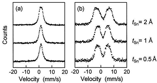
FIG. 5. ^{119}\text{Sn} Mössbauer spectra for (a) [\text{Fe}(10 \text{ \AA})/\text{Cr}(5 \text{ \AA})/\text{Sn}(t_{\text{Sn}})/\text{Cr}(5 \text{ \AA})] multilayers ( t_{\text{Sn}} = 2, 1, \text{ and } 0.5 \text{ \AA} ) and (b) [\text{Fe}(10 \text{ \AA})/\text{Cr}(22 \text{ \AA})/\text{Sn}(t_{\text{Sn}})/\text{Cr}(22 \text{ \AA})] multilayers ( t_{\text{Sn}} = 2, 1, \text{ and } 0.5 \text{ \AA} ) measured at 300 K.
