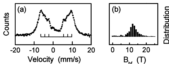
FIG. 1. (a) ^{119}\text{Sn} Mössbauer spectrum for [Cr(20 Å)/Sn(2 Å)] multilayer at 300 K. The peak positions for the magnetically split sextet are a guide to the eye. (b) The distribution of hyperfine field obtained from the fitting of the spectrum.
