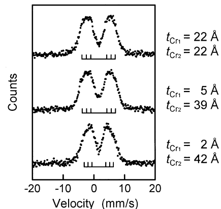
FIG. 4. ^{119}\text{Sn} Mössbauer spectra for [Fe(10 Å)/Cr( t_{\text{Cr}1} )/Sn(1 Å)/Cr( t_{\text{Cr}2} )] multilayers ( t_{\text{Cr}} = t_{\text{Cr}1} + t_{\text{Cr}2} = 44 Å, t_{\text{Cr}1} = 22, 5, and 2 Å) with the Sn layer in the different depth from the Fe/Cr interface at 300 K. The peak positions for the magnetically split sextet are a guide to the eye.
