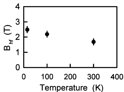
FIG. 3. Temperature dependence of the hyperfine field (at the maximum in distribution) for [Fe(10 Å)/Cr(5 Å)/Sn(2 Å)/Cr(5 Å)] multilayer obtained from the ^{119}\text{Sn} Mössbauer spectra.
