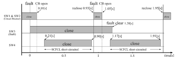
Fig. 4. Switching sequence for the repetitive operation test of SCFCLs.
