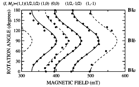
FIG. 2. Photoinduced STEL signals (closed circles) vs rotation angle measured at 8 K. Microwave frequency is 9.371( \pm 0.001 ) GHz. Magnetic-field vector \mathbf{B} is in the ab plane and the rotation axis is the c axis. (I, M_I) : the total nuclear spin of the STEL centers and the magnetic quantum number. Solid and dashed lines: fitting lines derived from the spin Hamiltonian described in Sec. IV A.
